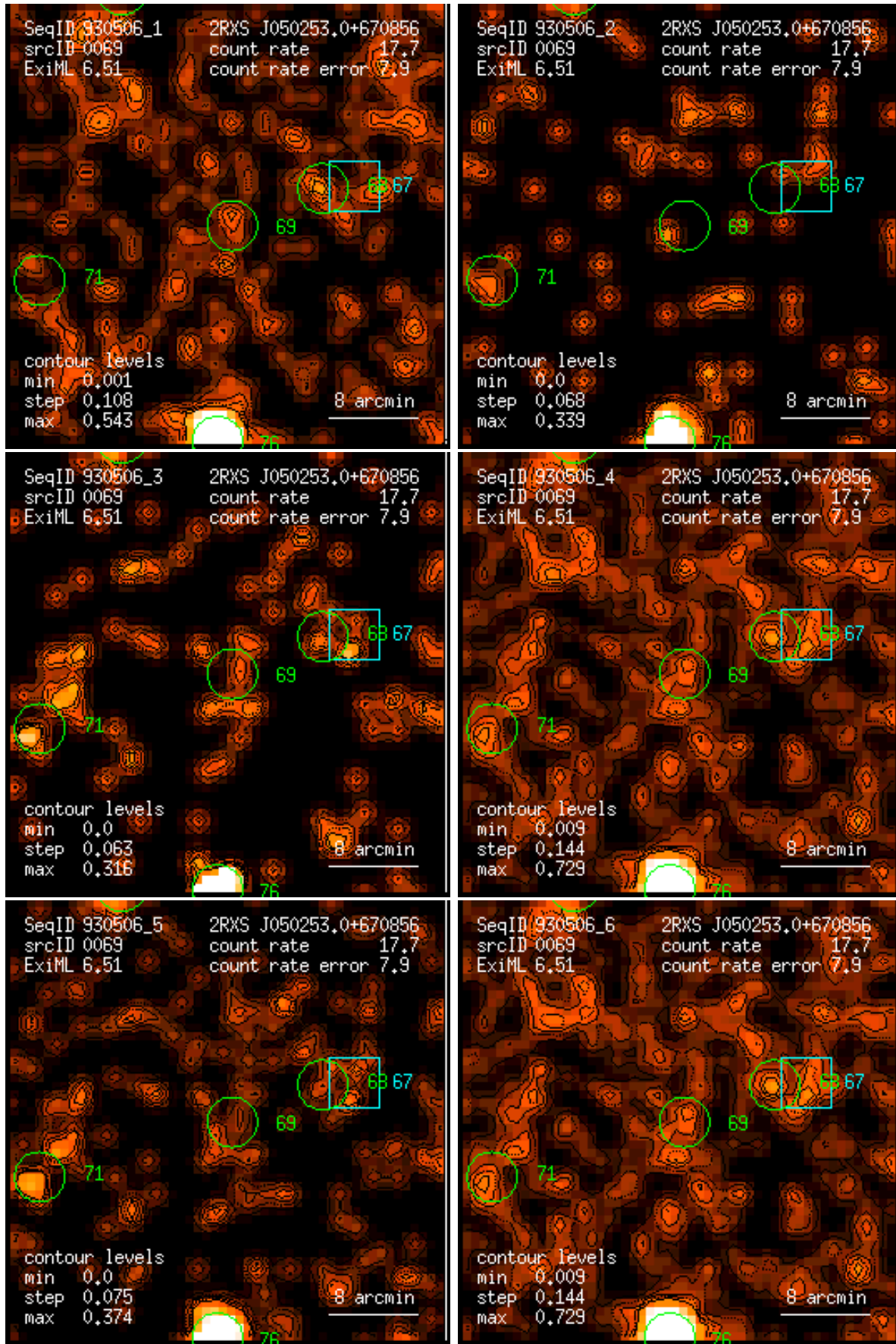
Figure 69: RASS 930506: detection 0069: band rate images, Gaussian filter: (1) PSPC channels 11 – 41, (2) 52 – 90, (3) 91 – 201, (4) 11 – 235, (5) 52 – 201, (6) 11 – 201. Broad band rates in counts/ks. Band rate contour levels in counts/ks/arcmin 2 .
