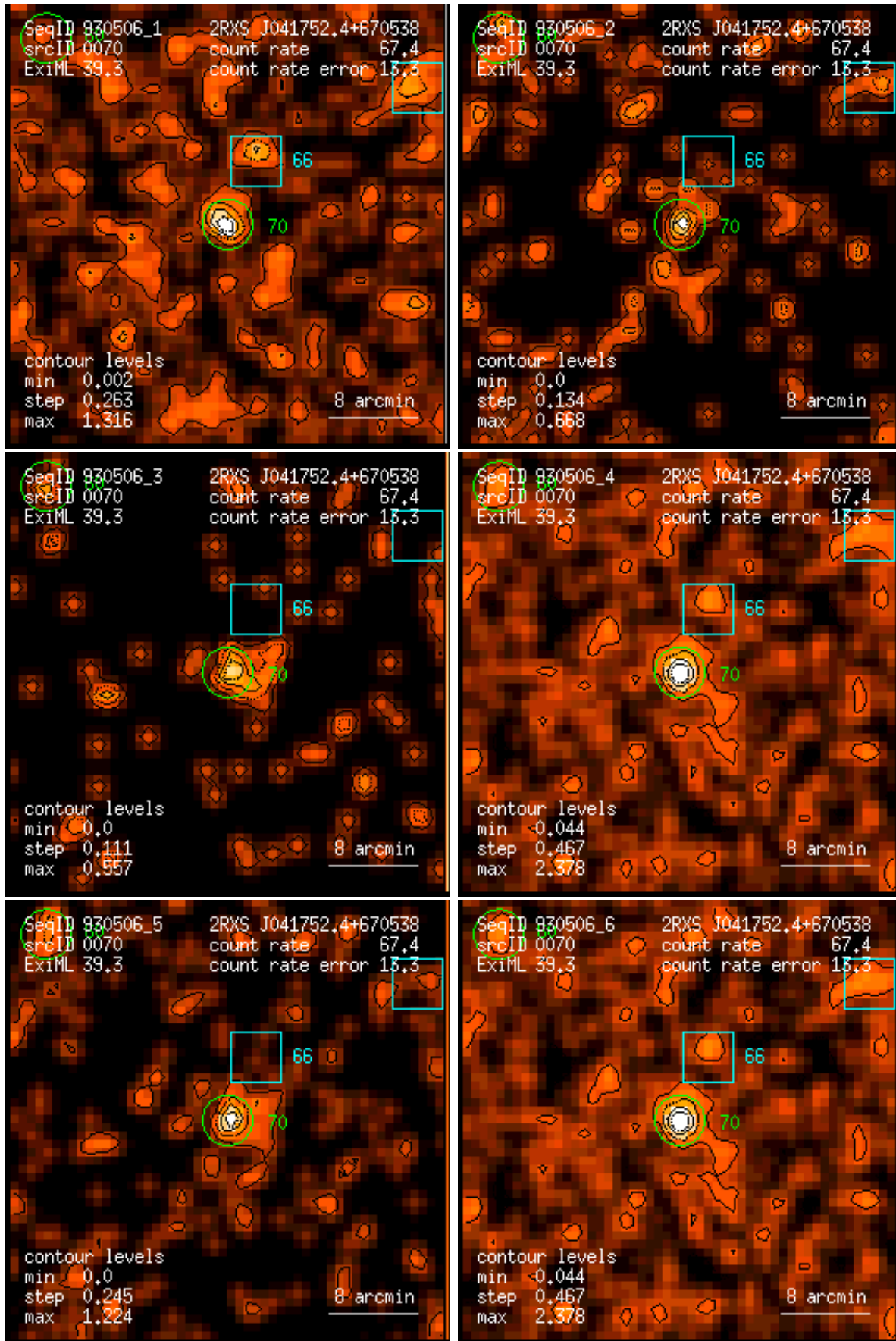
Figure 70: RASS 930506: detection 0070: band rate images, Gaussian filter: (1) PSPC channels 11 – 41, (2) 52 – 90, (3) 91 – 201, (4) 11 – 235, (5) 52 – 201, (6) 11 – 201. Broad band rates in counts/ks. Band rate contour levels in counts/ks/arcmin 2 .
