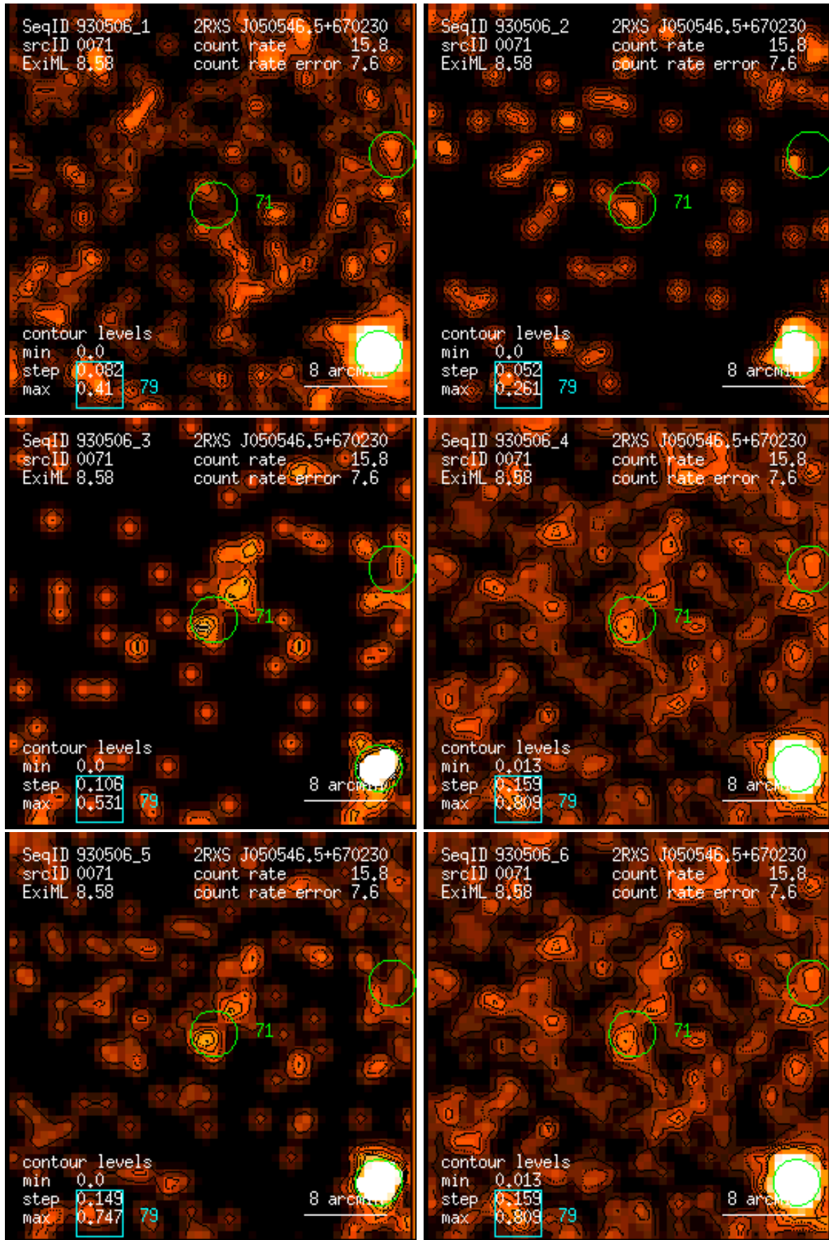
Figure 71: RASS 930506: detection 0071: band rate images, Gaussian filter: (1) PSPC channels 11 – 41, (2) 52 – 90, (3) 91 – 201, (4) 11 – 235, (5) 52 – 201, (6) 11 – 201. Broad band rates in counts/ks. Band rate contour levels in counts/ks/arcmin 2 .
