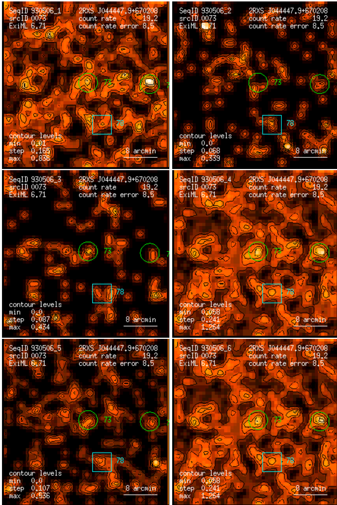
Figure 73: RASS 930506: detection 0073: band rate images, Gaussian filter: (1) PSPC channels 11 – 41, (2) 52 – 90, (3) 91 – 201, (4) 11 – 235, (5) 52 – 201, (6) 11 – 201. Broad band rates in counts/ks. Band rate contour levels in counts/ks/arcmin 2 .
