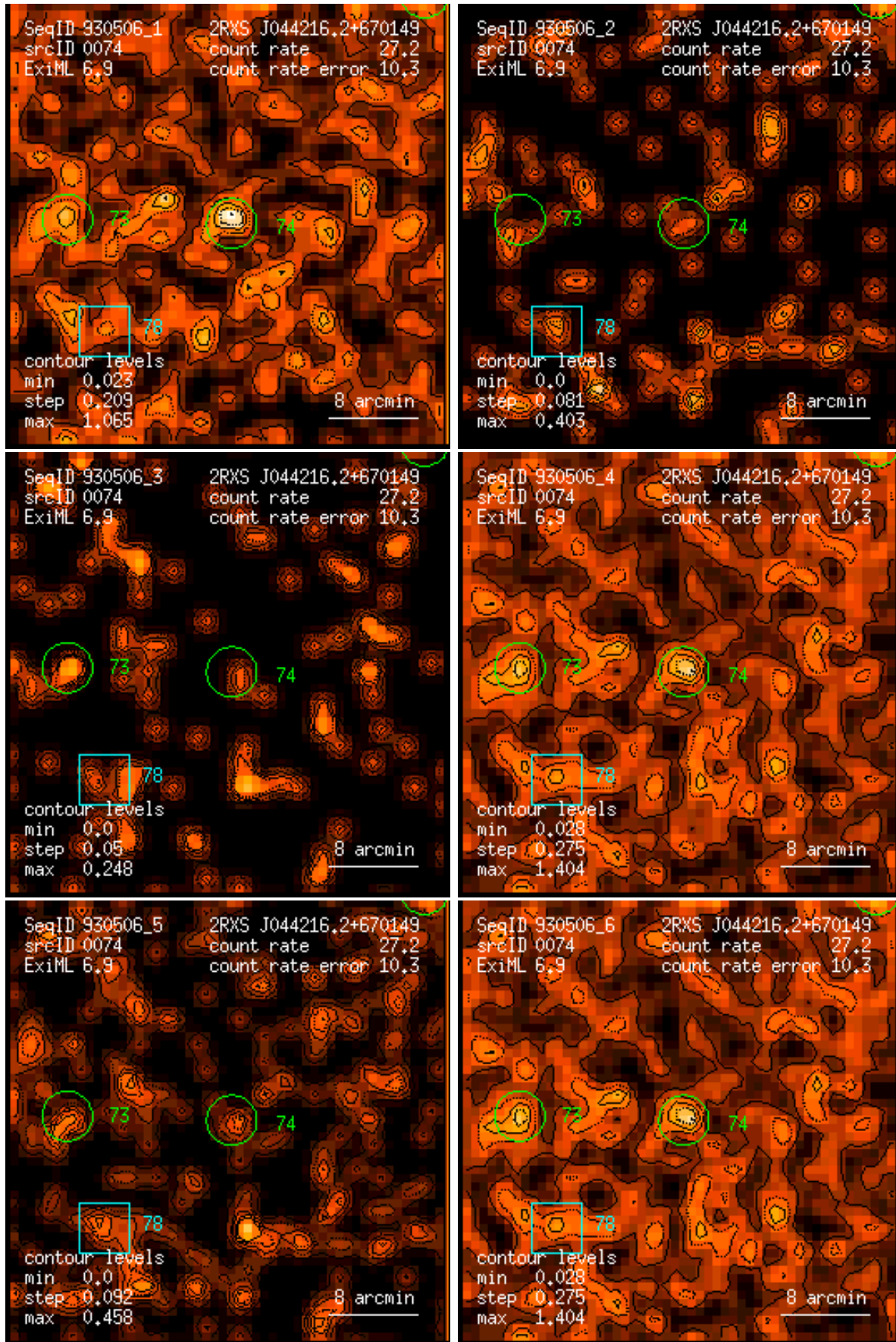
Figure 74: RASS 930506: detection 0074: band rate images, Gaussian filter: (1) PSPC channels 11 – 41, (2) 52 – 90, (3) 91 – 201, (4) 11 – 235, (5) 52 – 201, (6) 11 – 201. Broad band rates in counts/ks. Band rate contour levels in counts/ks/arcmin 2 .
