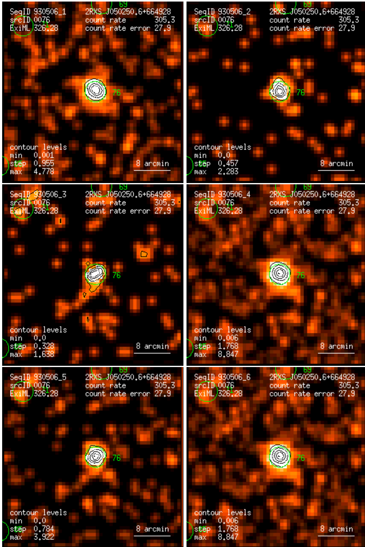
Figure 76: RASS 930506: detection 0076: band rate images, Gaussian filter: (1) PSPC channels 11 – 41, (2) 52 – 90, (3) 91 – 201, (4) 11 – 235, (5) 52 – 201, (6) 11 – 201. Broad band rates in counts/ks. Band rate contour levels in counts/ks/arcmin 2 .
