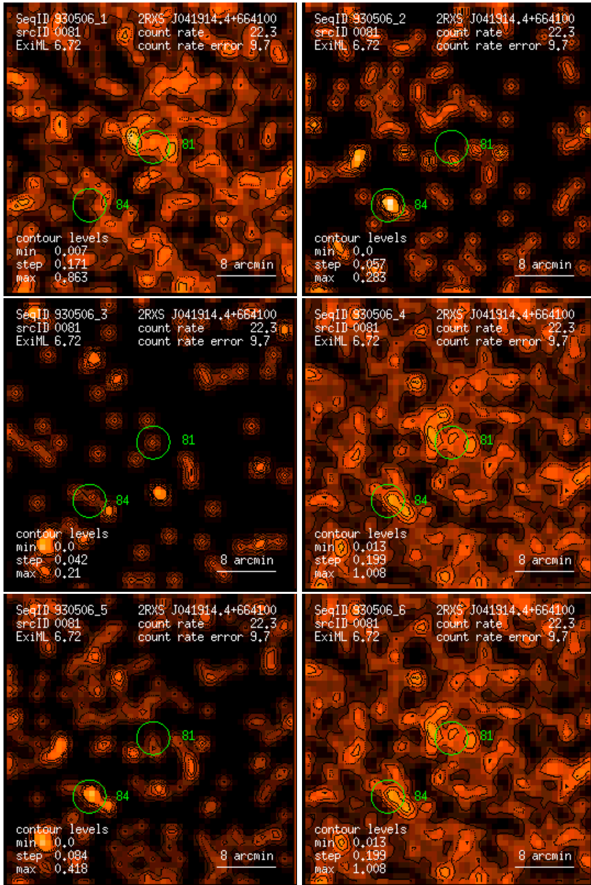
Figure 81: RASS 930506: detection 0081: band rate images, Gaussian filter: (1) PSPC channels 11 – 41, (2) 52 – 90, (3) 91 – 201, (4) 11 – 235, (5) 52 – 201, (6) 11 – 201. Broad band rates in counts/ks. Band rate contour levels in counts/ks/arcmin 2 .
