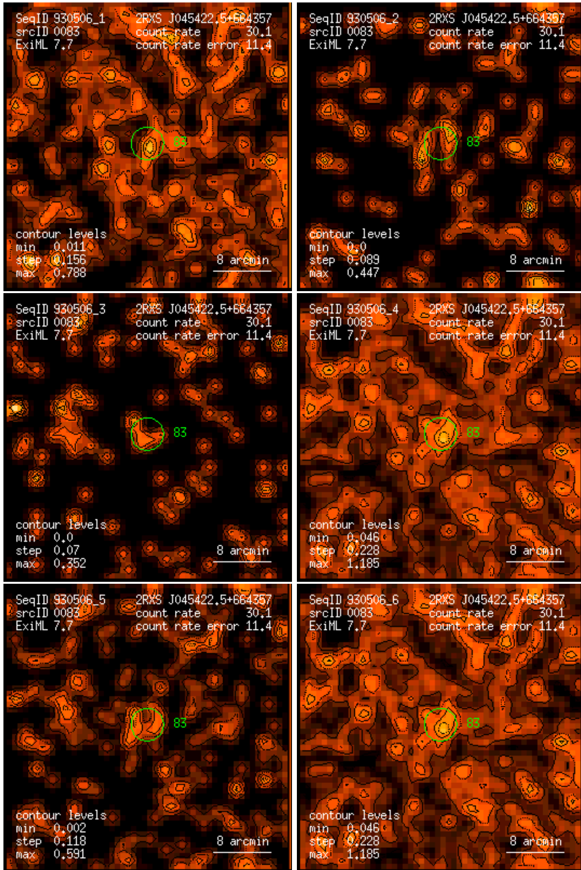
Figure 83: RASS 930506: detection 0083: band rate images, Gaussian filter: (1) PSPC channels 11 – 41, (2) 52 – 90, (3) 91 – 201, (4) 11 – 235, (5) 52 – 201, (6) 11 – 201. Broad band rates in counts/ks. Band rate contour levels in counts/ks/arcmin 2 .
