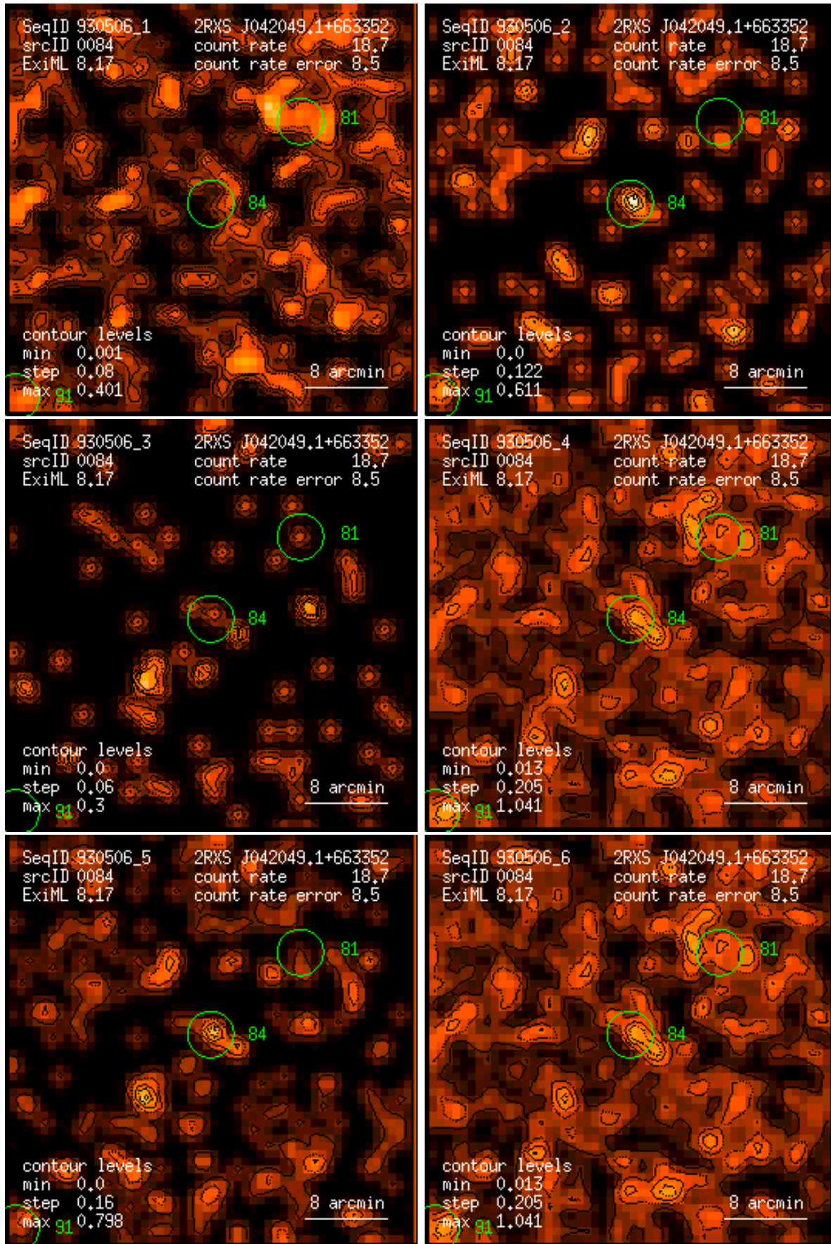
Figure 84: RASS 930506: detection 0084: band rate images, Gaussian filter: (1) PSPC channels 11 – 41, (2) 52 – 90, (3) 91 – 201, (4) 11 – 235, (5) 52 – 201, (6) 11 – 201. Broad band rates in counts/ks. Band rate contour levels in counts/ks/arcmin 2 .
