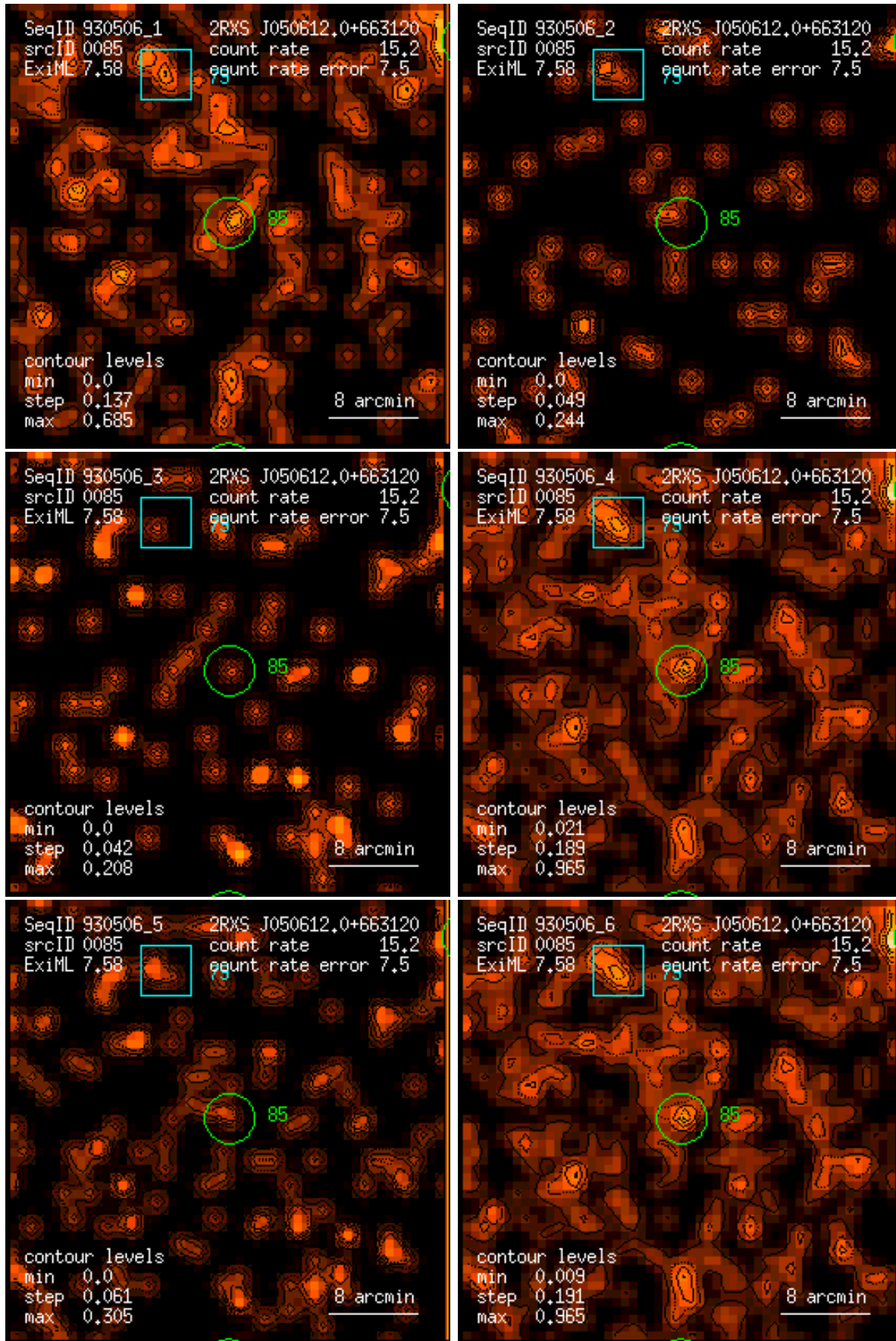
Figure 85: RASS 930506: detection 0085: band rate images, Gaussian filter: (1) PSPC channels 11 – 41, (2) 52 – 90, (3) 91 – 201, (4) 11 – 235, (5) 52 – 201, (6) 11 – 201. Broad band rates in counts/ks. Band rate contour levels in counts/ks/arcmin 2 .
