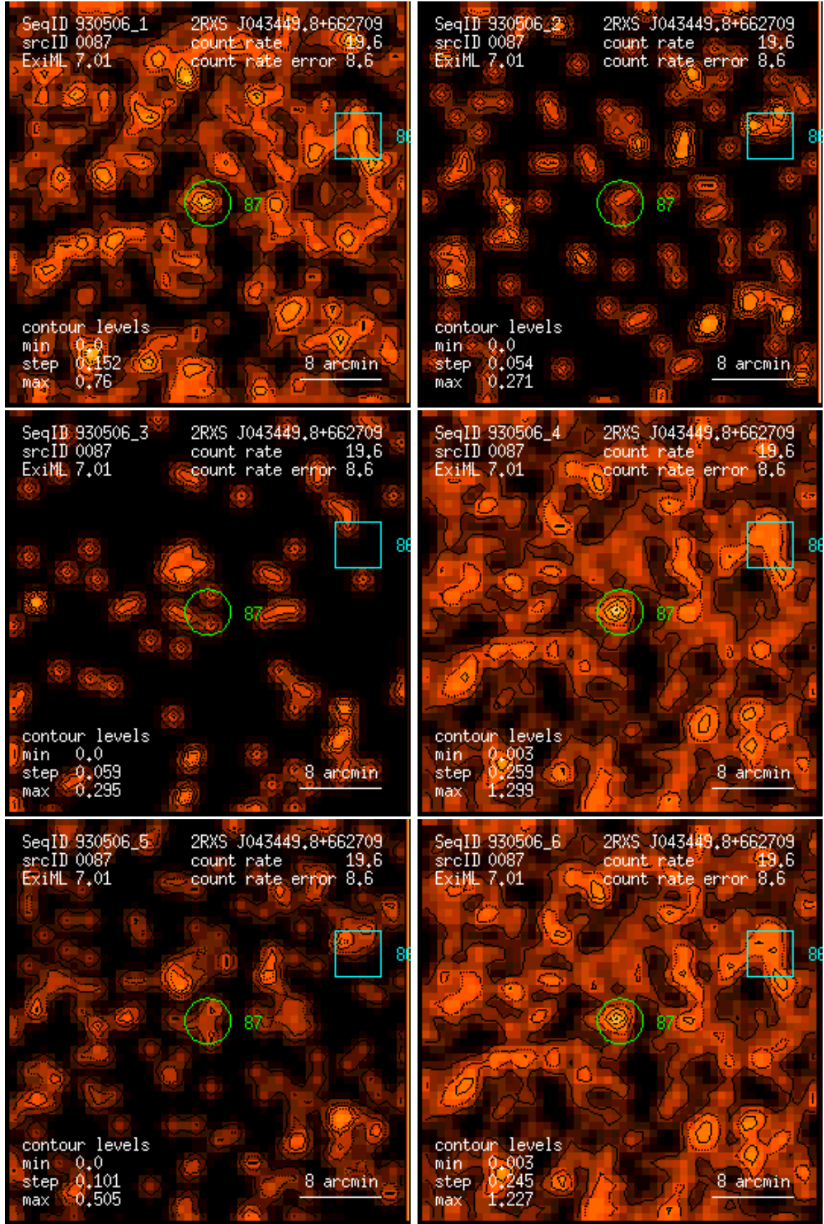
Figure 87: RASS 930506: detection 0087: band rate images, Gaussian filter: (1) PSPC channels 11 – 41, (2) 52 – 90, (3) 91 – 201, (4) 11 – 235, (5) 52 – 201, (6) 11 – 201. Broad band rates in counts/ks. Band rate contour levels in counts/ks/arcmin 2 .
