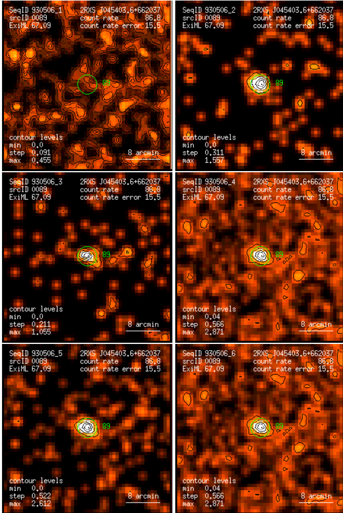
Figure 89: RASS 930506: detection 0089: band rate images, Gaussian filter: (1) PSPC channels 11 – 41, (2) 52 – 90, (3) 91 – 201, (4) 11 – 235, (5) 52 – 201, (6) 11 – 201. Broad band rates in counts/ks. Band rate contour levels in counts/ks/arcmin 2 .
