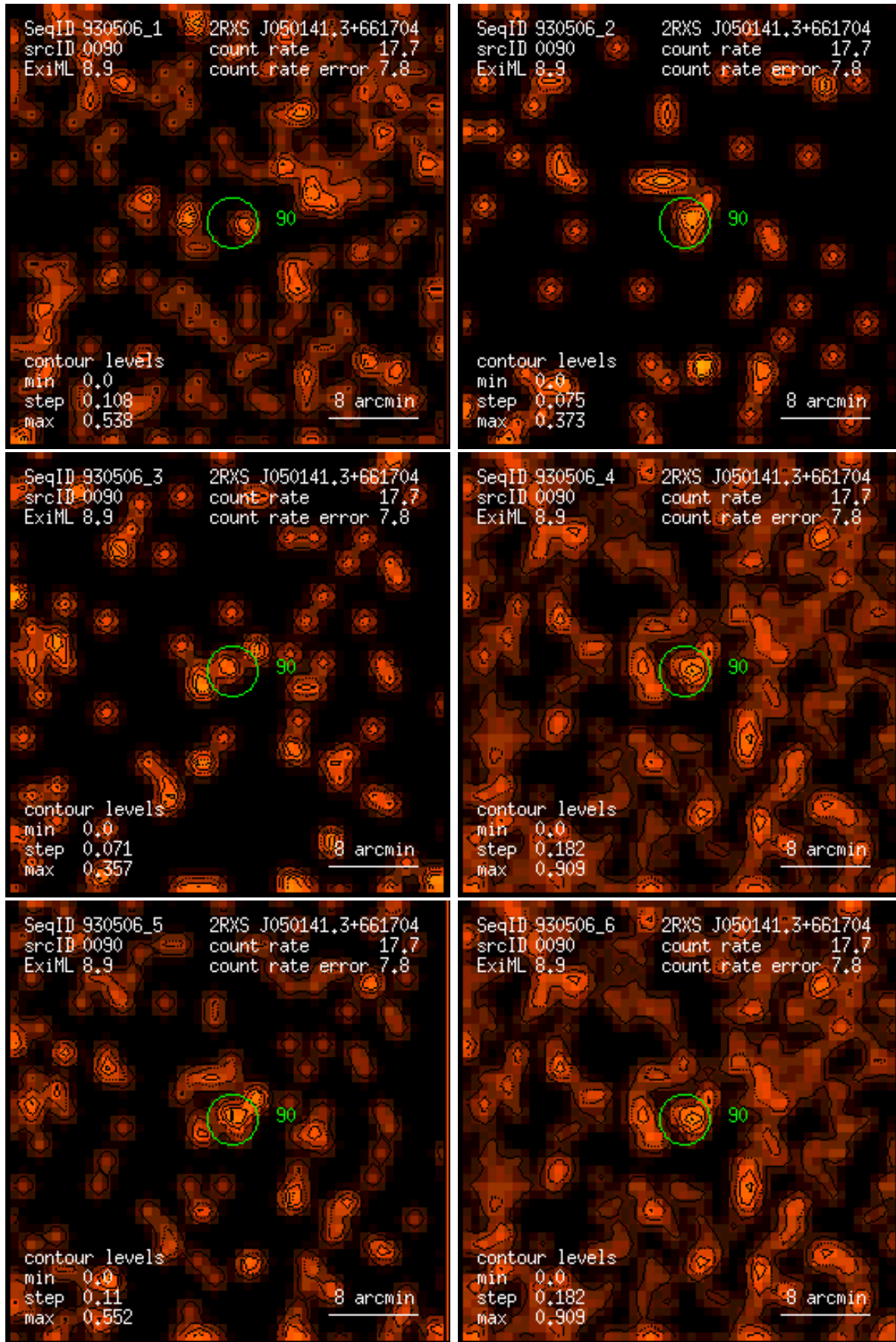
Figure 90: RASS 930506: detection 0090: band rate images, Gaussian filter: (1) PSPC channels 11 – 41, (2) 52 – 90, (3) 91 – 201, (4) 11 – 235, (5) 52 – 201, (6) 11 – 201. Broad band rates in counts/ks. Band rate contour levels in counts/ks/arcmin 2 .
