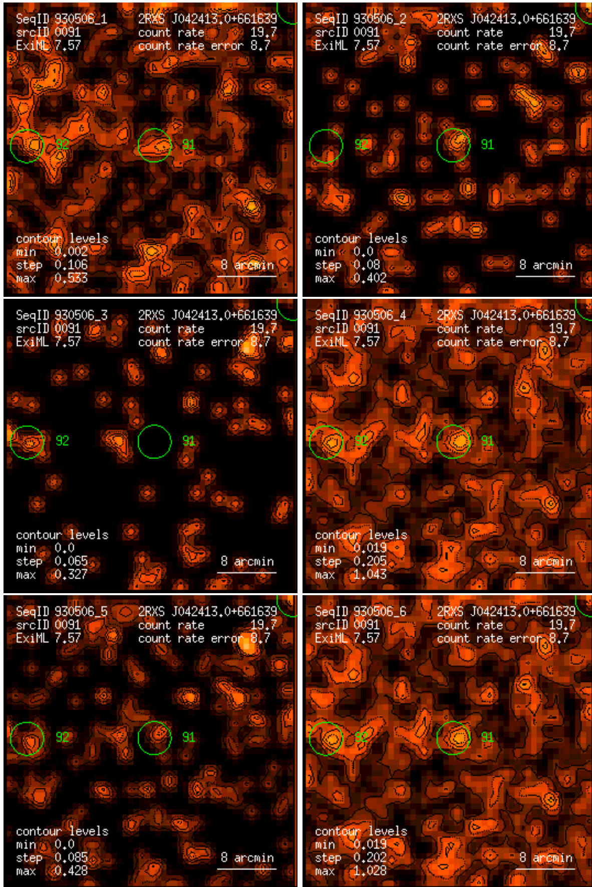
Figure 91: RASS 930506: detection 0091: band rate images, Gaussian filter: (1) PSPC channels 11 – 41, (2) 52 – 90, (3) 91 – 201, (4) 11 – 235, (5) 52 – 201, (6) 11 – 201. Broad band rates in counts/ks. Band rate contour levels in counts/ks/arcmin 2 .
