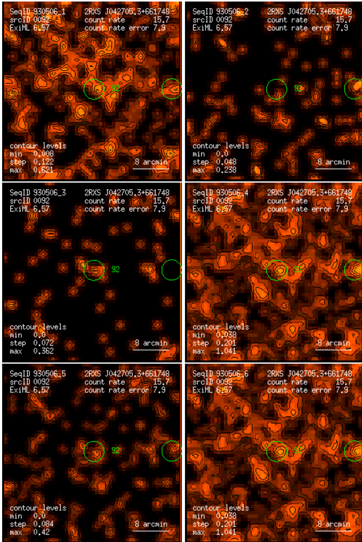
Figure 92: RASS 930506: detection 0092: band rate images, Gaussian filter: (1) PSPC channels 11 – 41, (2) 52 – 90, (3) 91 – 201, (4) 11 – 235, (5) 52 – 201, (6) 11 – 201. Broad band rates in counts/ks. Band rate contour levels in counts/ks/arcmin 2 .
