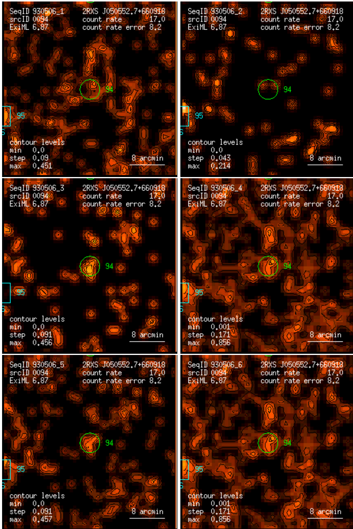
Figure 94: RASS 930506: detection 0094: band rate images, Gaussian filter: (1) PSPC channels 11 – 41, (2) 52 – 90, (3) 91 – 201, (4) 11 – 235, (5) 52 – 201, (6) 11 – 201. Broad band rates in counts/ks. Band rate contour levels in counts/ks/arcmin 2 .
