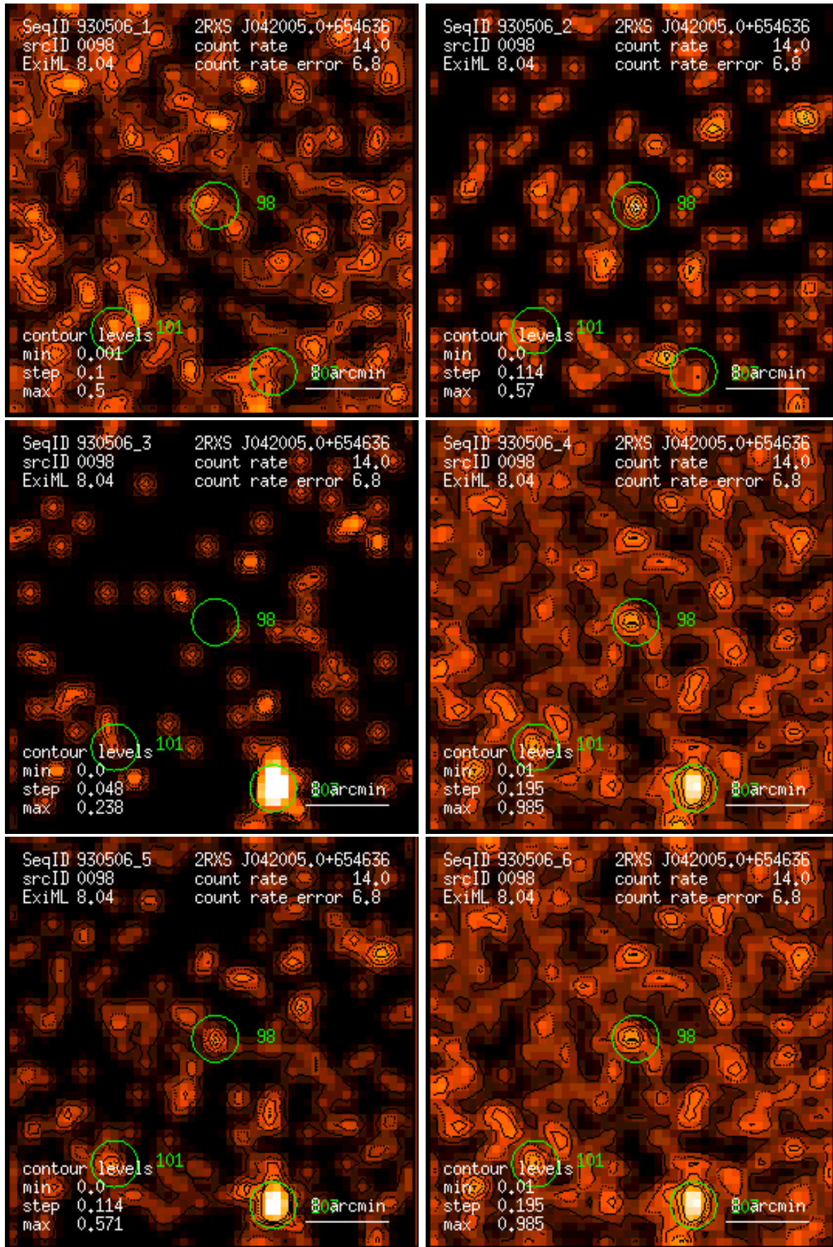
Figure 98: RASS 930506: detection 0098: band rate images, Gaussian filter: (1) PSPC channels 11 – 41, (2) 52 – 90, (3) 91 – 201, (4) 11 – 235, (5) 52 – 201, (6) 11 – 201. Broad band rates in counts/ks. Band rate contour levels in counts/ks/arcmin 2 .
