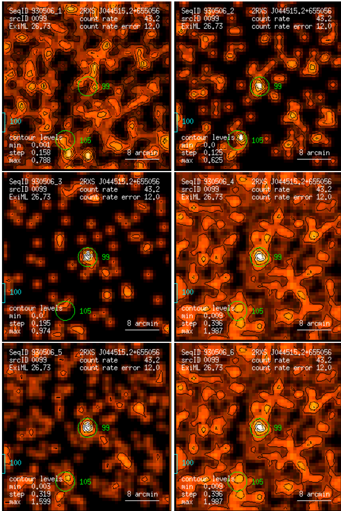
Figure 99: RASS 930506: detection 0099: band rate images, Gaussian filter: (1) PSPC channels 11 – 41, (2) 52 – 90, (3) 91 – 201, (4) 11 – 235, (5) 52 – 201, (6) 11 – 201. Broad band rates in counts/ks. Band rate contour levels in counts/ks/arcmin 2 .
