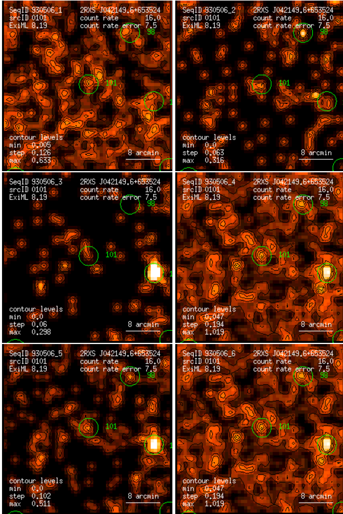
Figure 101: RASS 930506: detection 0101: band rate images, Gaussian filter: (1) PSPC channels 11 – 41, (2) 52 – 90, (3) 91 – 201, (4) 11 – 235, (5) 52 – 201, (6) 11 – 201. Broad band rates in counts/ks. Band rate contour levels in counts/ks/arcmin 2 .
