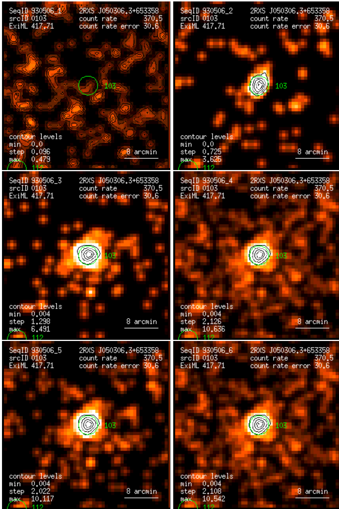
Figure 103: RASS 930506: detection 0103: band rate images, Gaussian filter: (1) PSPC channels 11 – 41, (2) 52 – 90, (3) 91 – 201, (4) 11 – 235, (5) 52 – 201, (6) 11 – 201. Broad band rates in counts/ks. Band rate contour levels in counts/ks/arcmin 2 .
