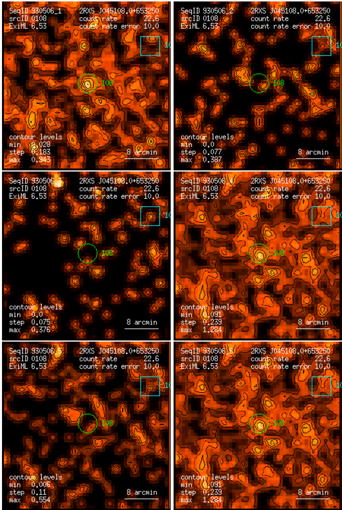
Figure 108: RASS 930506: detection 0108: band rate images, Gaussian filter: (1) PSPC channels 11 – 41, (2) 52 – 90, (3) 91 – 201, (4) 11 – 235, (5) 52 – 201, (6) 11 – 201. Broad band rates in counts/ks. Band rate contour levels in counts/ks/arcmin 2 .
