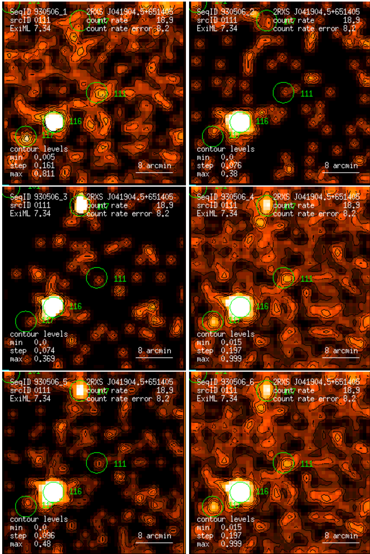
Figure 111: RASS 930506: detection 0111: band rate images, Gaussian filter: (1) PSPC channels 11 – 41, (2) 52 – 90, (3) 91 – 201, (4) 11 – 235, (5) 52 – 201, (6) 11 – 201. Broad band rates in counts/ks. Band rate contour levels in counts/ks/arcmin 2 .
