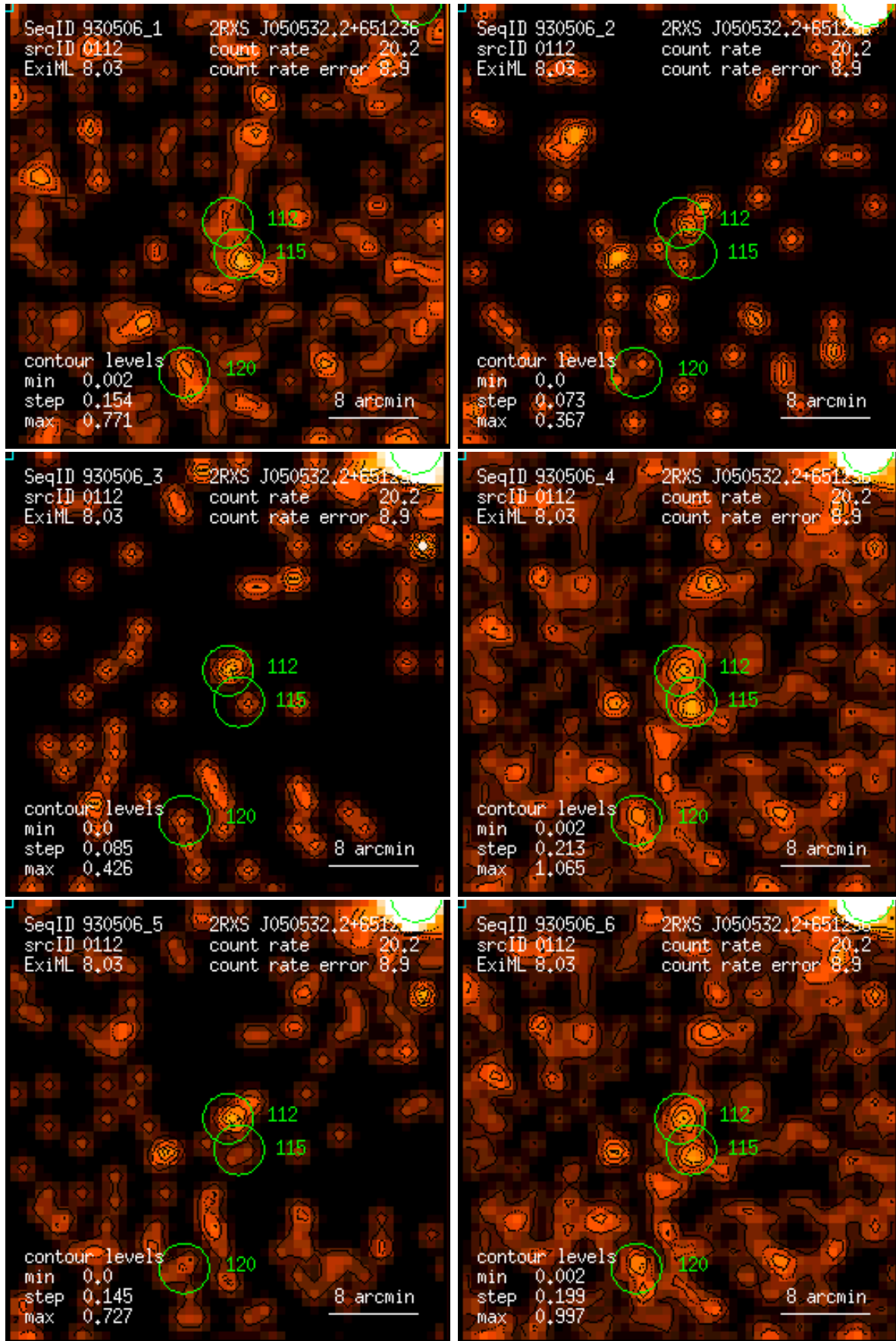
Figure 112: RASS 930506: detection 0112: band rate images, Gaussian filter: (1) PSPC channels 11 – 41, (2) 52 – 90, (3) 91 – 201, (4) 11 – 235, (5) 52 – 201, (6) 11 – 201. Broad band rates in counts/ks. Band rate contour levels in counts/ks/arcmin 2 .
