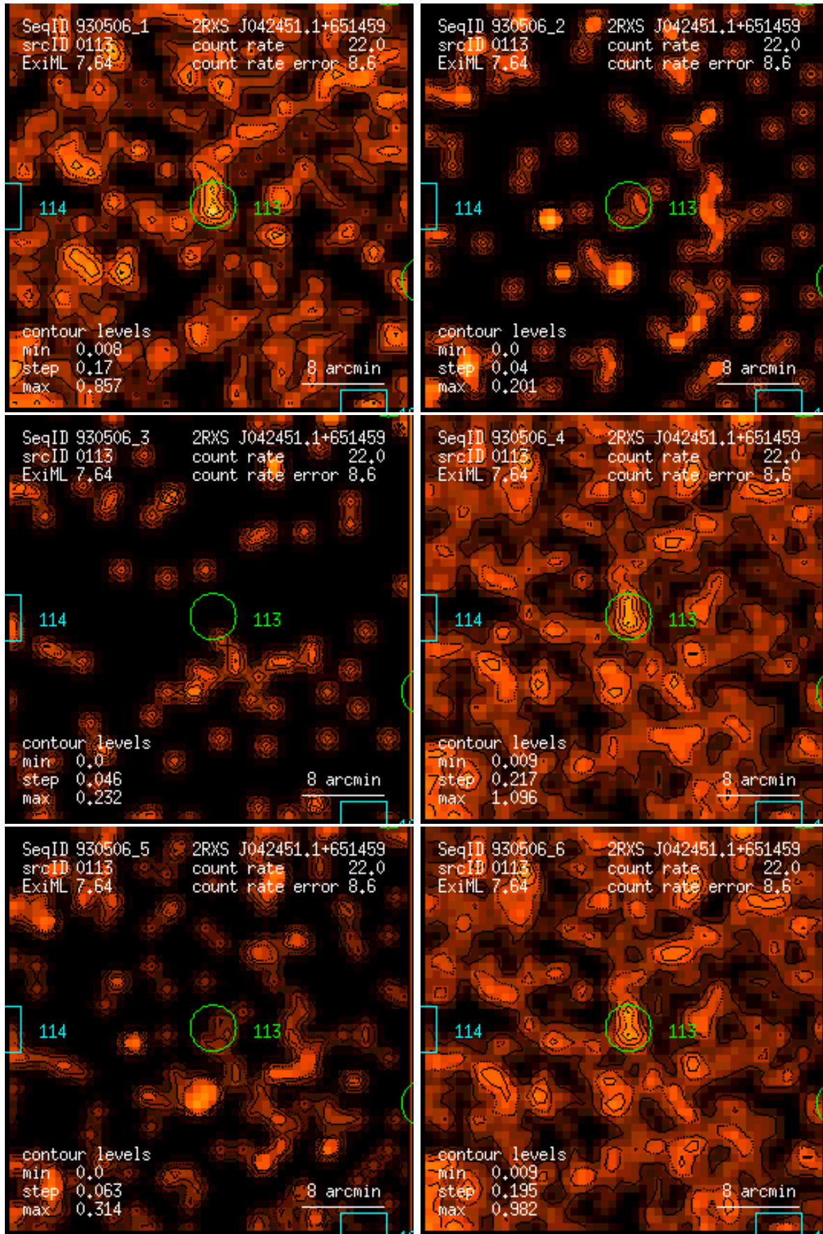
Figure 113: RASS 930506: detection 0113: band rate images, Gaussian filter: (1) PSPC channels 11 – 41, (2) 52 – 90, (3) 91 – 201, (4) 11 – 235, (5) 52 – 201, (6) 11 – 201. Broad band rates in counts/ks. Band rate contour levels in counts/ks/arcmin 2 .
