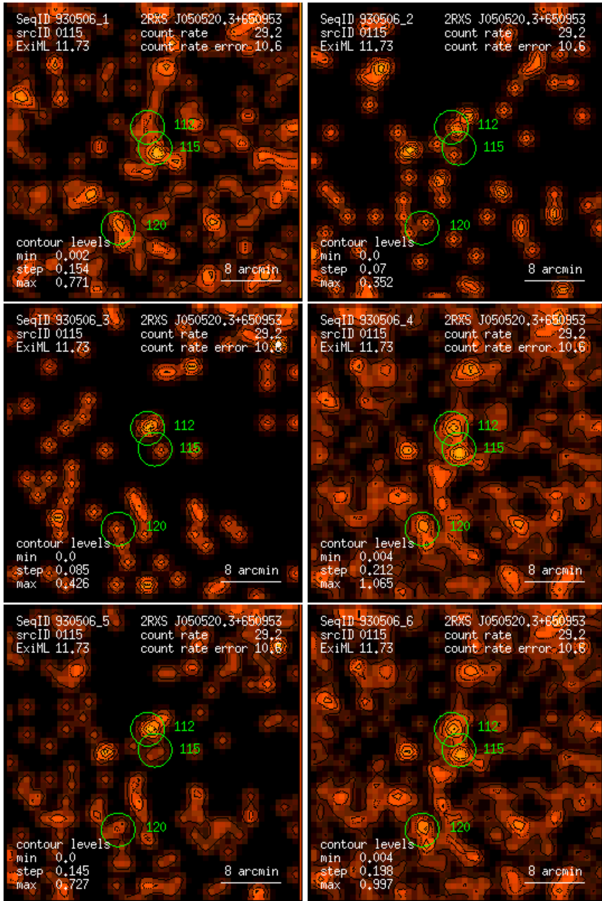
Figure 115: RASS 930506: detection 0115: band rate images, Gaussian filter: (1) PSPC channels 11 – 41, (2) 52 – 90, (3) 91 – 201, (4) 11 – 235, (5) 52 – 201, (6) 11 – 201. Broad band rates in counts/ks. Band rate contour levels in counts/ks/arcmin 2 .
