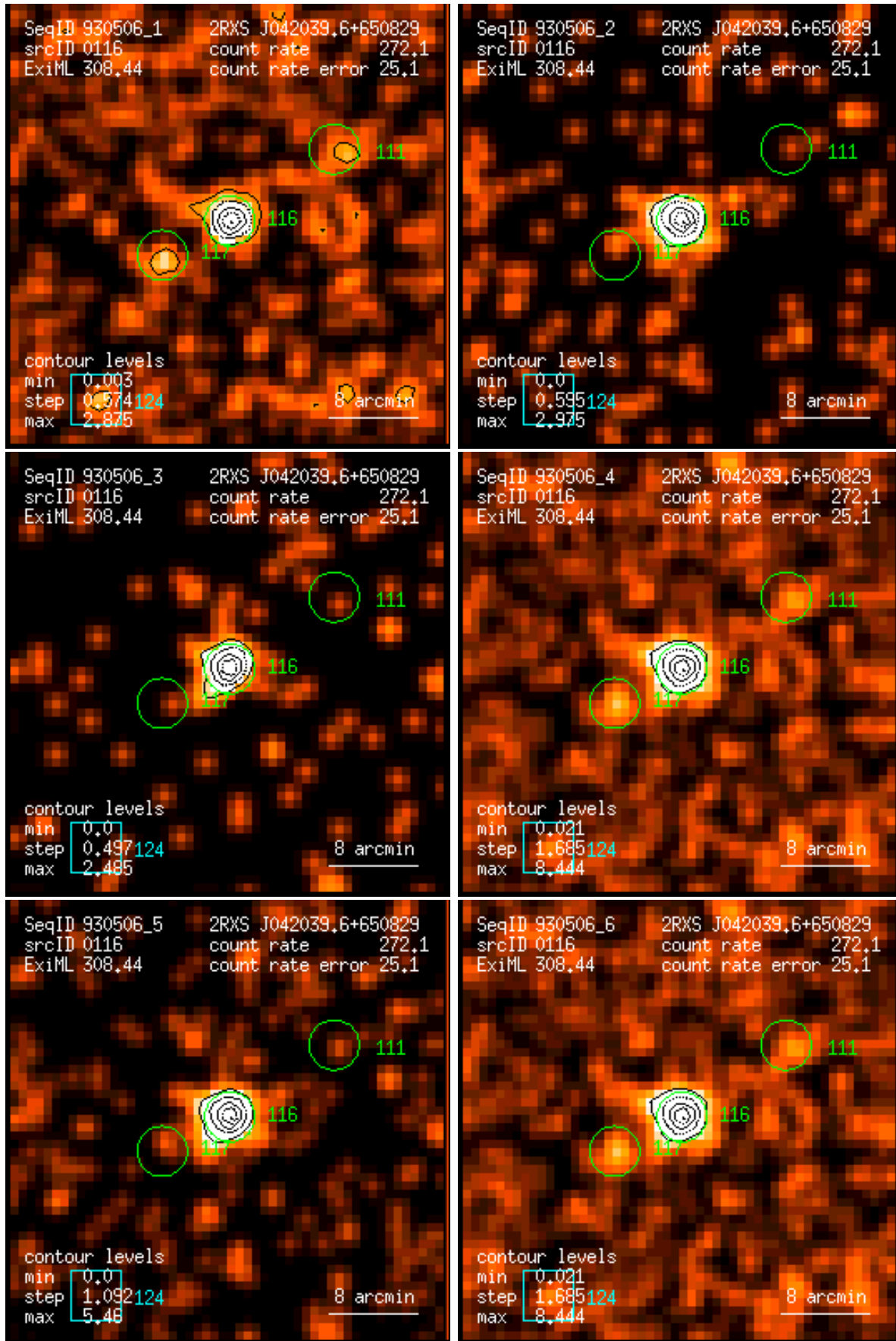
Figure 116: RASS 930506: detection 0116: band rate images, Gaussian filter: (1) PSPC channels 11 – 41, (2) 52 – 90, (3) 91 – 201, (4) 11 – 235, (5) 52 – 201, (6) 11 – 201. Broad band rates in counts/ks. Band rate contour levels in counts/ks/arcmin 2 .
