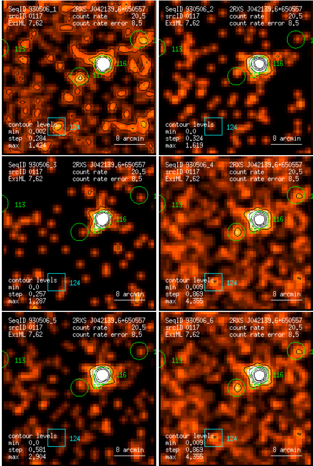
Figure 117: RASS 930506: detection 0117: band rate images, Gaussian filter: (1) PSPC channels 11 – 41, (2) 52 – 90, (3) 91 – 201, (4) 11 – 235, (5) 52 – 201, (6) 11 – 201. Broad band rates in counts/ks. Band rate contour levels in counts/ks/arcmin 2 .
