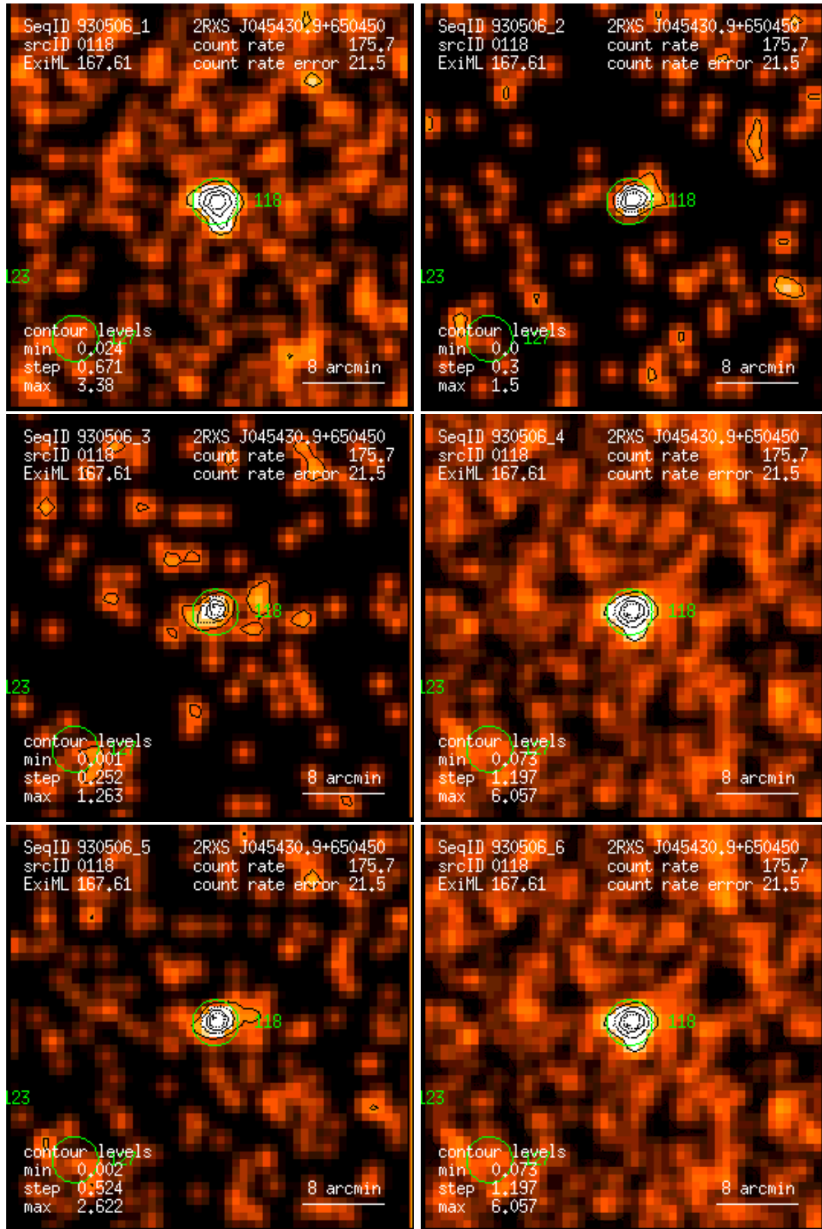
Figure 118: RASS 930506: detection 0118: band rate images, Gaussian filter: (1) PSPC channels 11 – 41, (2) 52 – 90, (3) 91 – 201, (4) 11 – 235, (5) 52 – 201, (6) 11 – 201. Broad band rates in counts/ks. Band rate contour levels in counts/ks/arcmin 2 .
