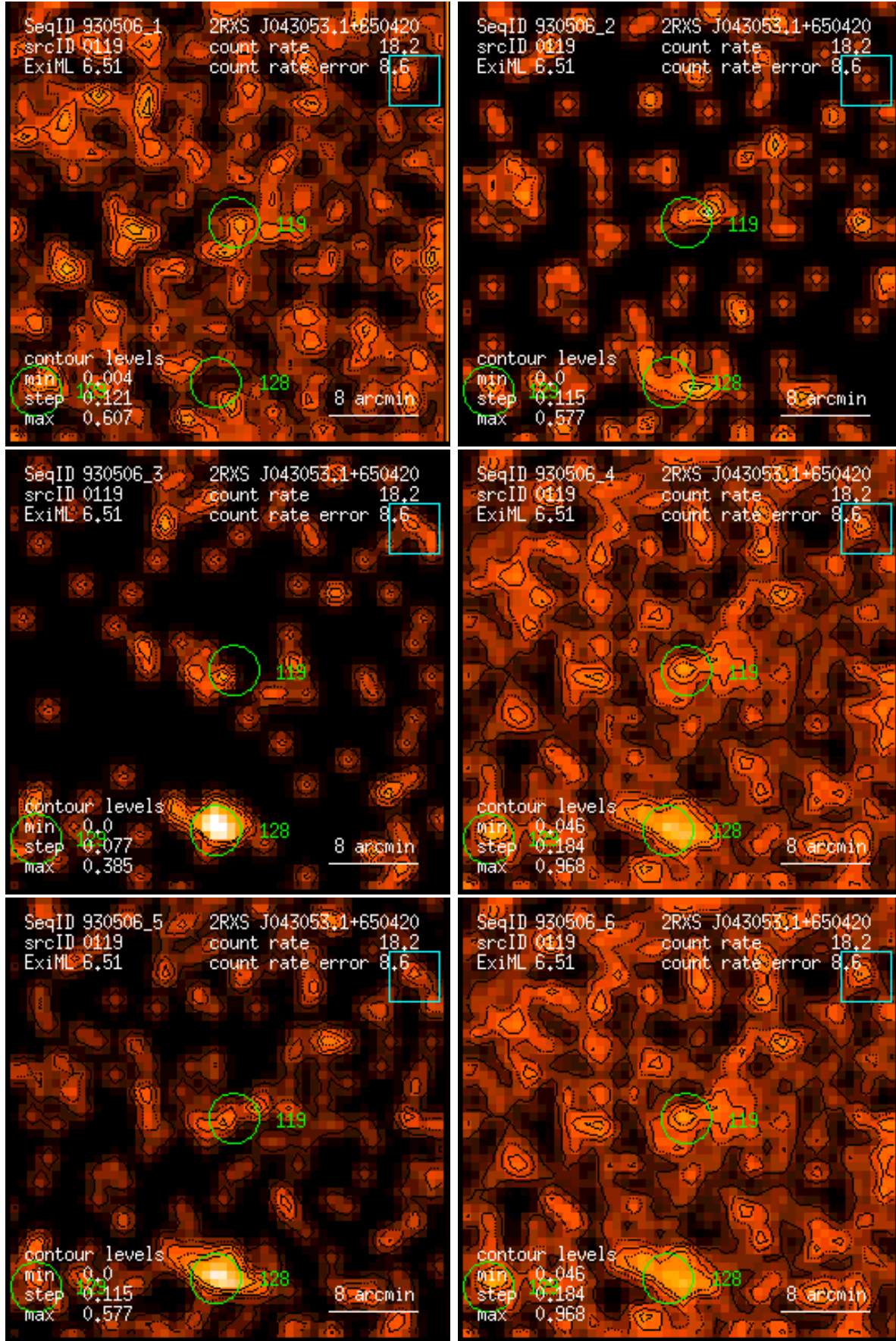
Figure 119: RASS 930506: detection 0119: band rate images, Gaussian filter: (1) PSPC channels 11 – 41, (2) 52 – 90, (3) 91 – 201, (4) 11 – 235, (5) 52 – 201, (6) 11 – 201. Broad band rates in counts/ks. Band rate contour levels in counts/ks/arcmin 2 .
