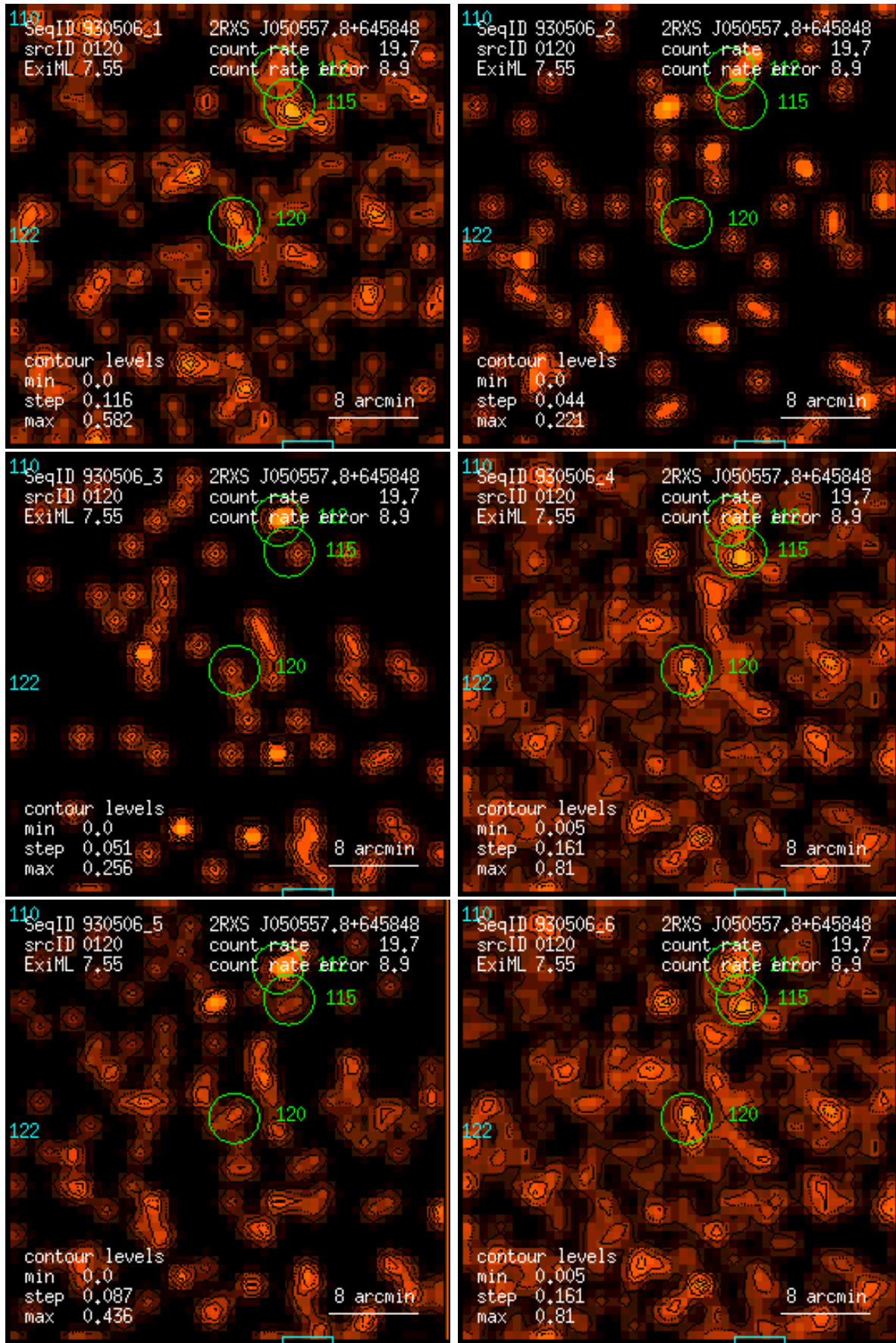
Figure 120: RASS 930506: detection 0120: band rate images, Gaussian filter: (1) PSPC channels 11 – 41, (2) 52 – 90, (3) 91 – 201, (4) 11 – 235, (5) 52 – 201, (6) 11 – 201. Broad band rates in counts/ks. Band rate contour levels in counts/ks/arcmin 2 .
