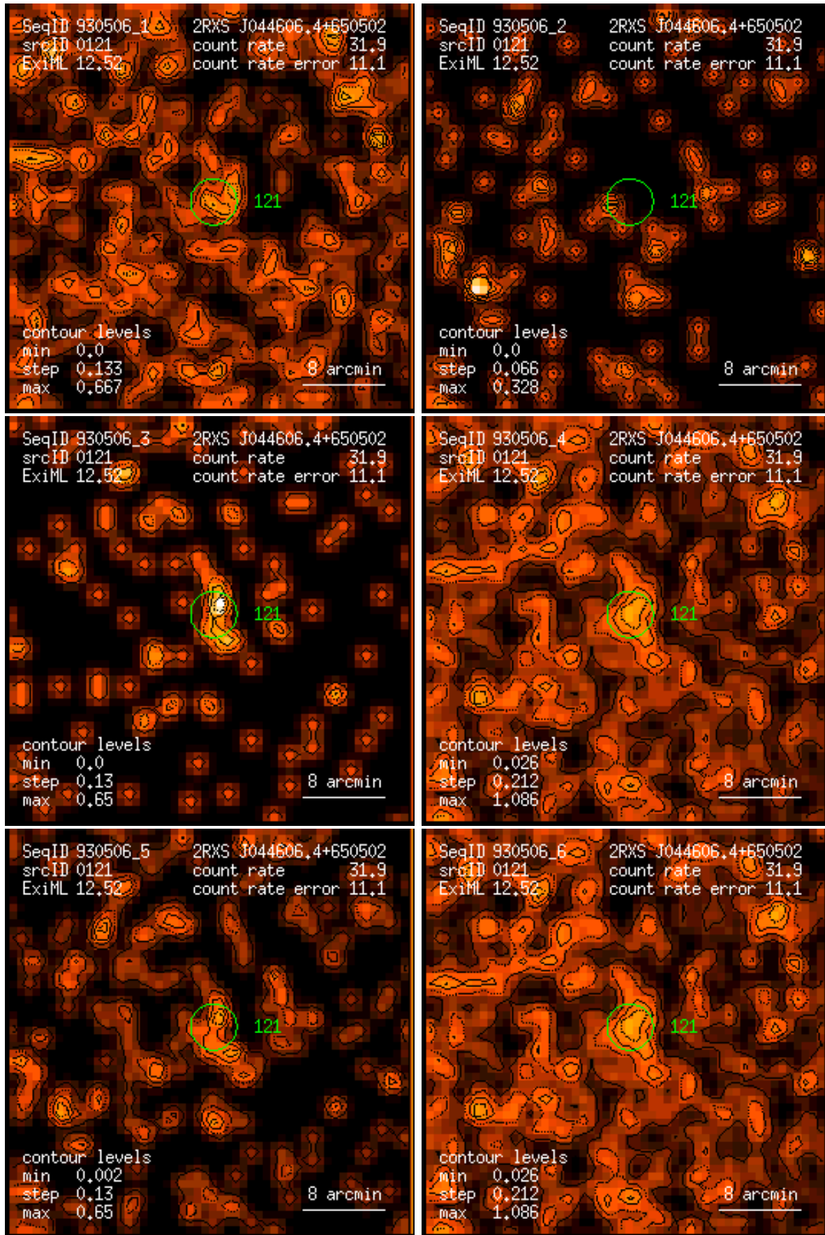
Figure 121: RASS 930506: detection 0121: band rate images, Gaussian filter: (1) PSPC channels 11 – 41, (2) 52 – 90, (3) 91 – 201, (4) 11 – 235, (5) 52 – 201, (6) 11 – 201. Broad band rates in counts/ks. Band rate contour levels in counts/ks/arcmin 2 .
