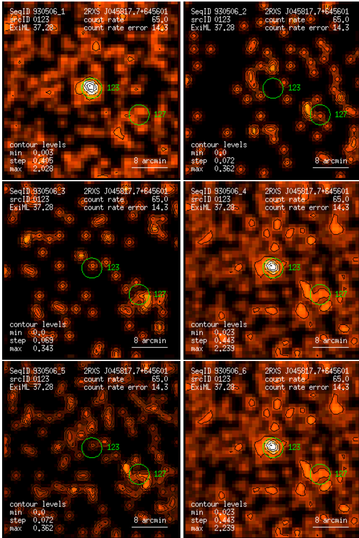
Figure 123: RASS 930506: detection 0123: band rate images, Gaussian filter: (1) PSPC channels 11 – 41, (2) 52 – 90, (3) 91 – 201, (4) 11 – 235, (5) 52 – 201, (6) 11 – 201. Broad band rates in counts/ks. Band rate contour levels in counts/ks/arcmin 2 .
