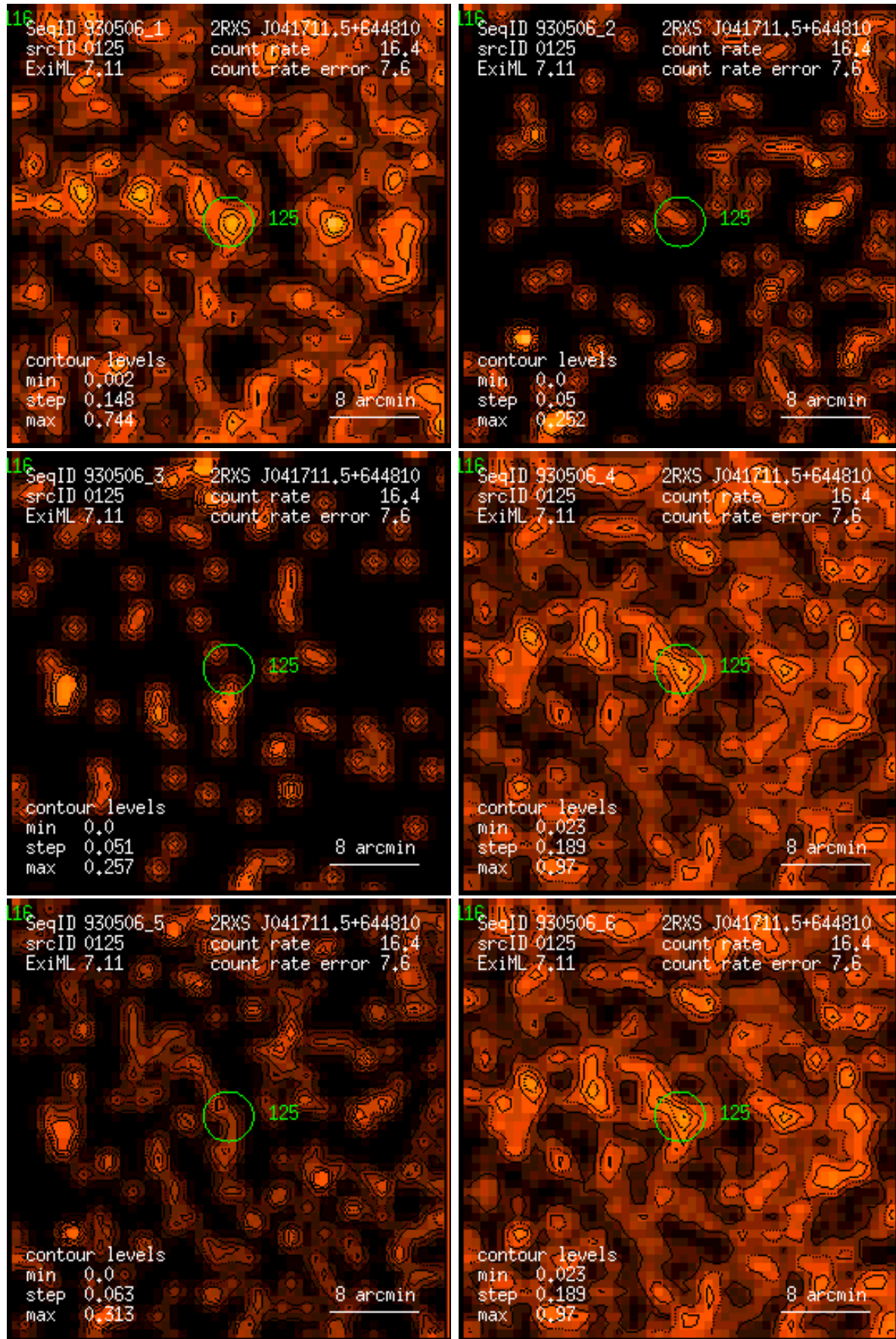
Figure 125: RASS 930506: detection 0125: band rate images, Gaussian filter: (1) PSPC channels 11 – 41, (2) 52 – 90, (3) 91 – 201, (4) 11 – 235, (5) 52 – 201, (6) 11 – 201. Broad band rates in counts/ks. Band rate contour levels in counts/ks/arcmin 2 .
