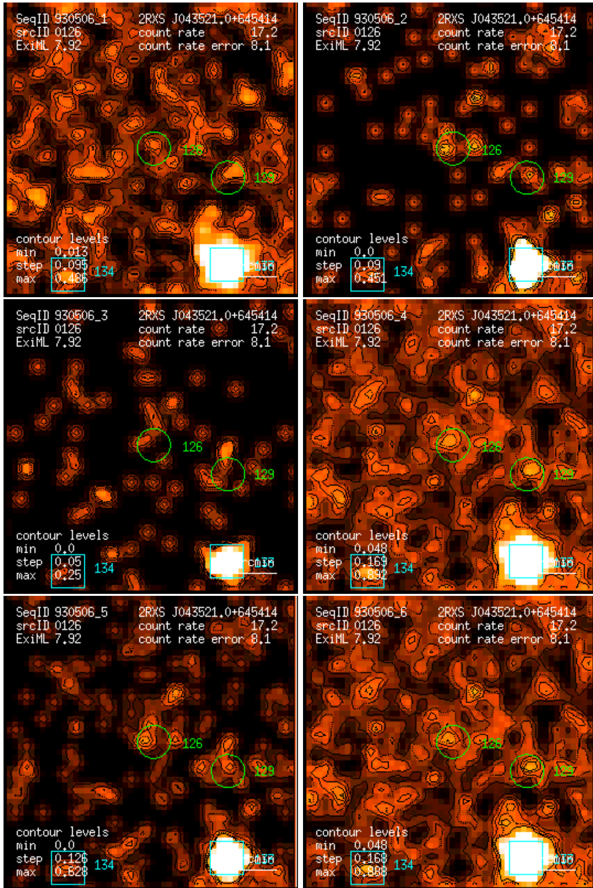
Figure 126: RASS 930506: detection 0126: band rate images, Gaussian filter: (1) PSPC channels 11 – 41, (2) 52 – 90, (3) 91 – 201, (4) 11 – 235, (5) 52 – 201, (6) 11 – 201. Broad band rates in counts/ks. Band rate contour levels in counts/ks/arcmin 2 .
