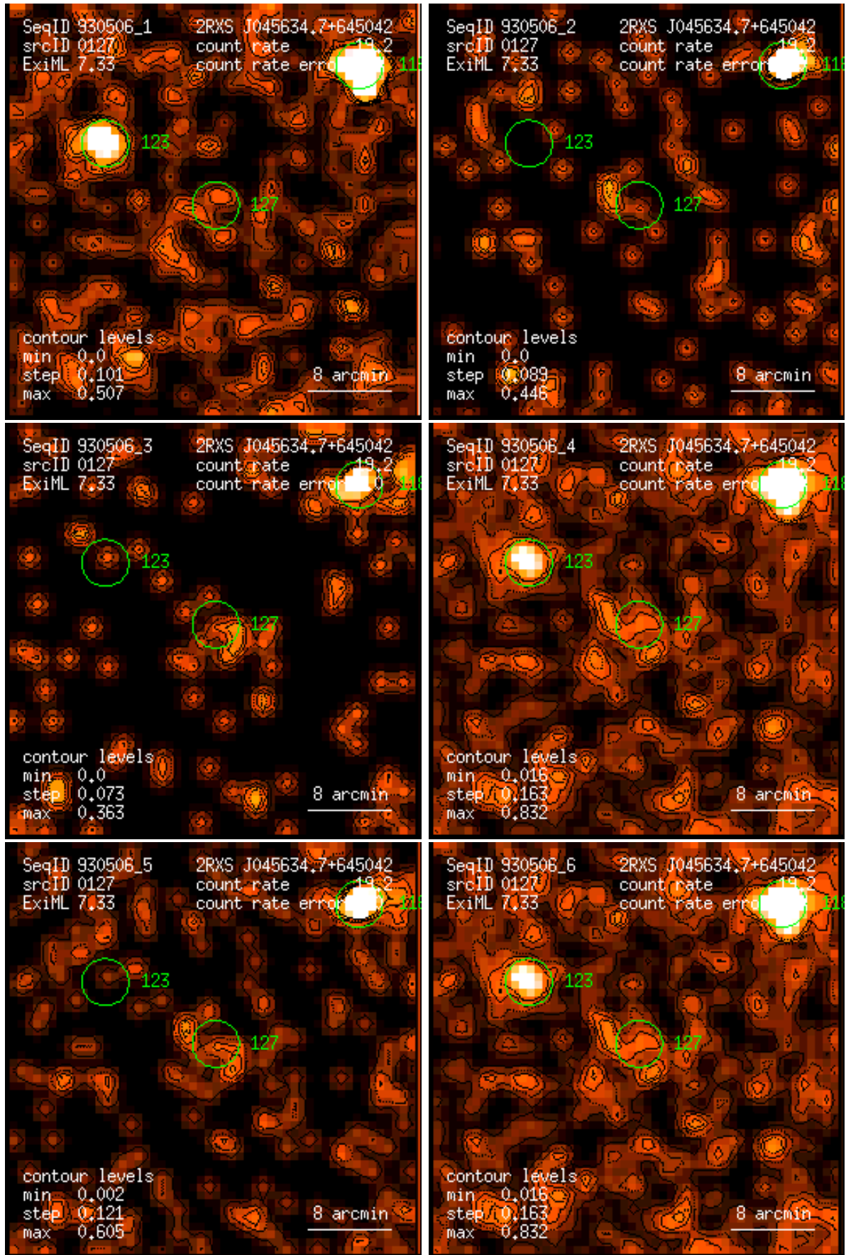
Figure 127: RASS 930506: detection 0127: band rate images, Gaussian filter: (1) PSPC channels 11 – 41, (2) 52 – 90, (3) 91 – 201, (4) 11 – 235, (5) 52 – 201, (6) 11 – 201. Broad band rates in counts/ks. Band rate contour levels in counts/ks/arcmin 2 .
