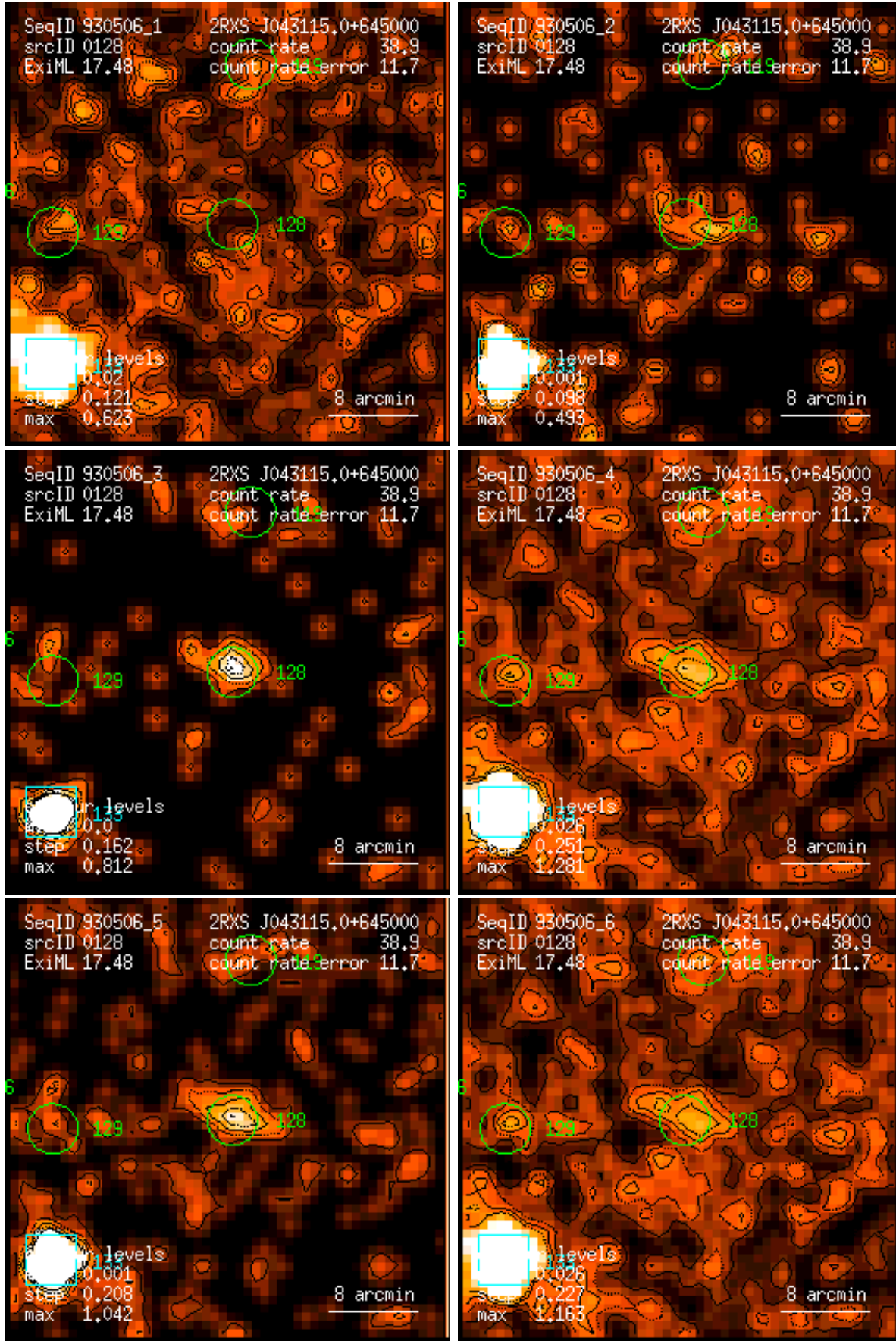
Figure 128: RASS 930506: detection 0128: band rate images, Gaussian filter: (1) PSPC channels 11 – 41, (2) 52 – 90, (3) 91 – 201, (4) 11 – 235, (5) 52 – 201, (6) 11 – 201. Broad band rates in counts/ks. Band rate contour levels in counts/ks/arcmin 2 .
