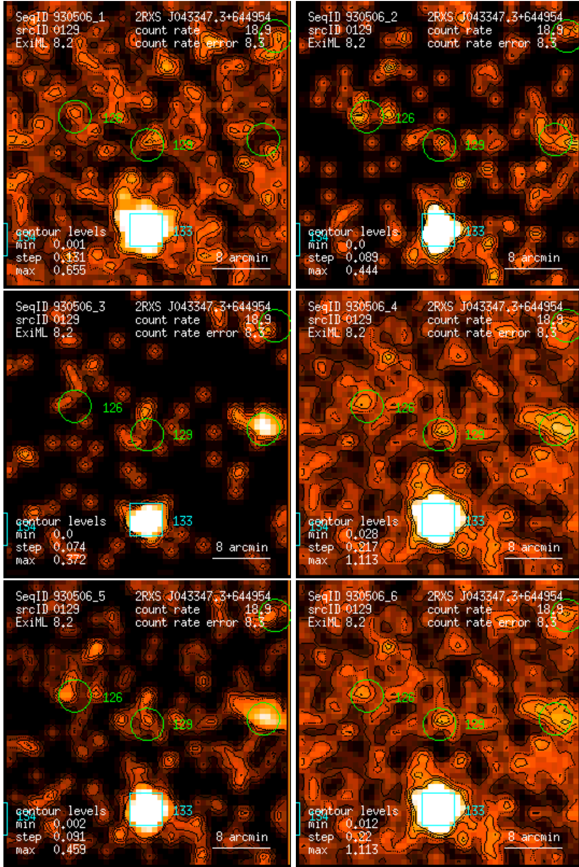
Figure 129: RASS 930506: detection 0129: band rate images, Gaussian filter: (1) PSPC channels 11 – 41, (2) 52 – 90, (3) 91 – 201, (4) 11 – 235, (5) 52 – 201, (6) 11 – 201. Broad band rates in counts/ks. Band rate contour levels in counts/ks/arcmin 2 .
