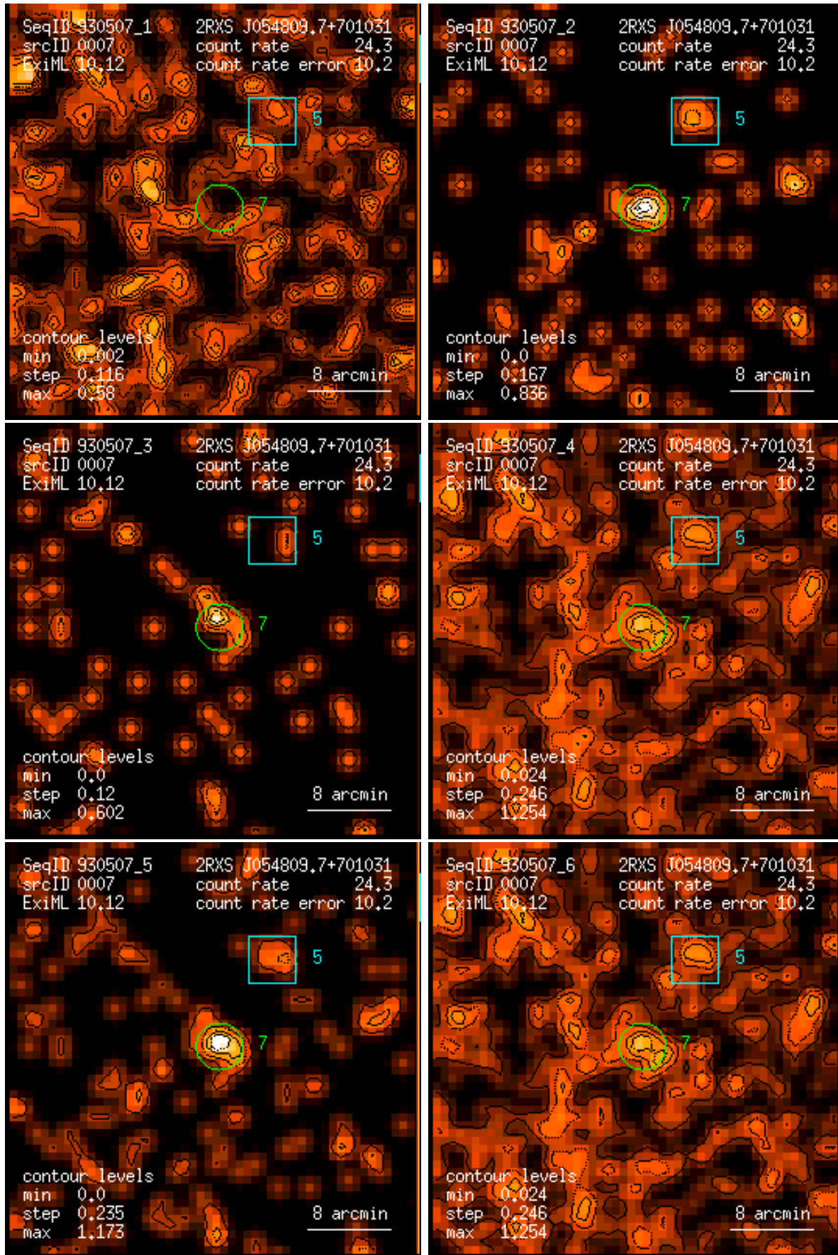
Figure 7: RASS 930507: detection 0007: band rate images, Gaussian filter: (1) PSPC channels 11 – 41, (2) 52 – 90, (3) 91 – 201, (4) 11 – 235, (5) 52 – 201, (6) 11 – 201. Broad band rates in counts/ks. Band rate contour levels in counts/ks/arcmin 2 .
