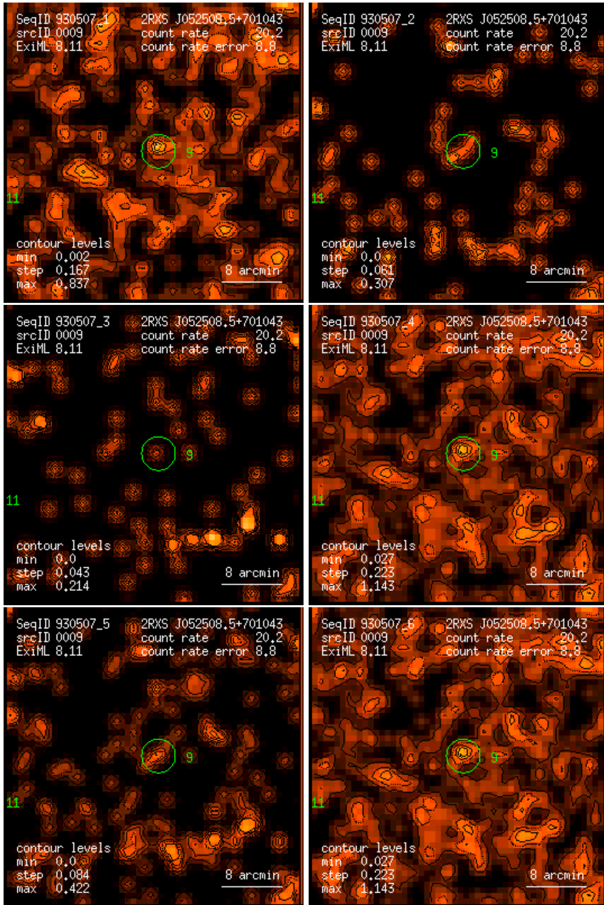
Figure 9: RASS 930507: detection 0009: band rate images, Gaussian filter: (1) PSPC channels 11 – 41, (2) 52 – 90, (3) 91 – 201, (4) 11 – 235, (5) 52 – 201, (6) 11 – 201. Broad band rates in counts/ks. Band rate contour levels in counts/ks/arcmin 2 .
