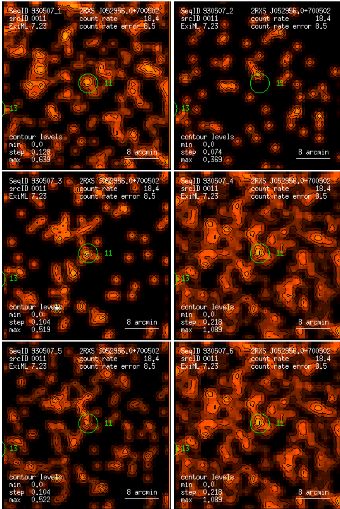
Figure 11: RASS 930507: detection 0011: band rate images, Gaussian filter: (1) PSPC channels 11 – 41, (2) 52 – 90, (3) 91 – 201, (4) 11 – 235, (5) 52 – 201, (6) 11 – 201. Broad band rates in counts/ks. Band rate contour levels in counts/ks/arcmin 2 .
