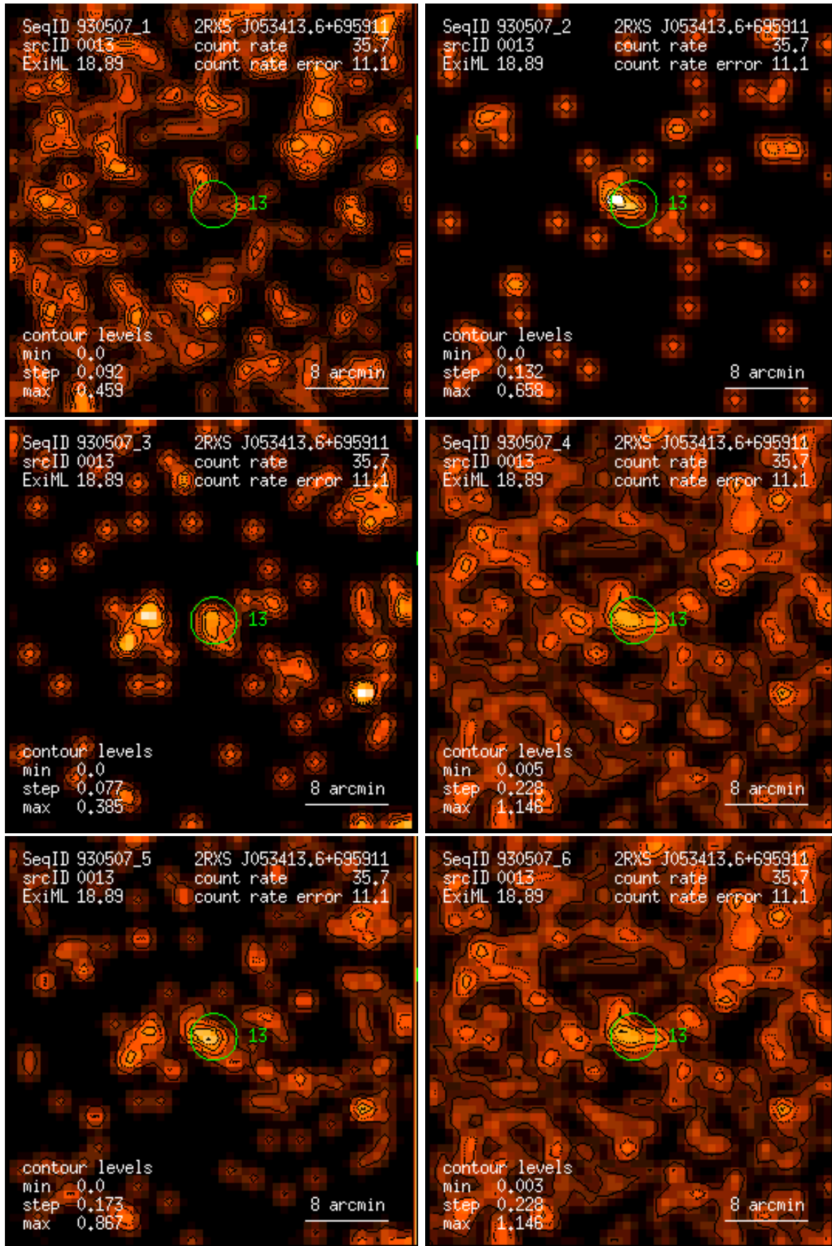
Figure 13: RASS 930507: detection 0013: band rate images, Gaussian filter: (1) PSPC channels 11 – 41, (2) 52 – 90, (3) 91 – 201, (4) 11 – 235, (5) 52 – 201, (6) 11 – 201. Broad band rates in counts/ks. Band rate contour levels in counts/ks/arcmin 2 .
