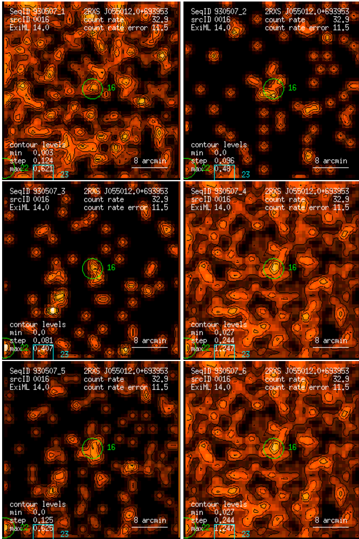
Figure 16: RASS 930507: detection 0016: band rate images, Gaussian filter: (1) PSPC channels 11 – 41, (2) 52 – 90, (3) 91 – 201, (4) 11 – 235, (5) 52 – 201, (6) 11 – 201. Broad band rates in counts/ks. Band rate contour levels in counts/ks/arcmin 2 .
