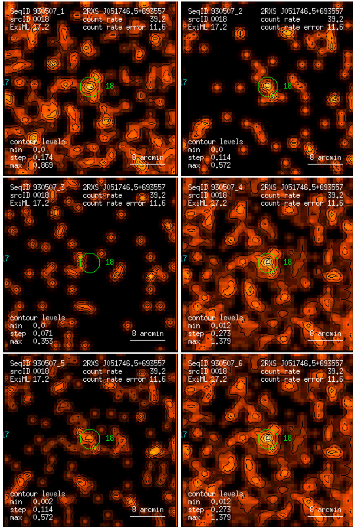
Figure 18: RASS 930507: detection 0018: band rate images, Gaussian filter: (1) PSPC channels 11 – 41, (2) 52 – 90, (3) 91 – 201, (4) 11 – 235, (5) 52 – 201, (6) 11 – 201. Broad band rates in counts/ks. Band rate contour levels in counts/ks/arcmin 2 .
