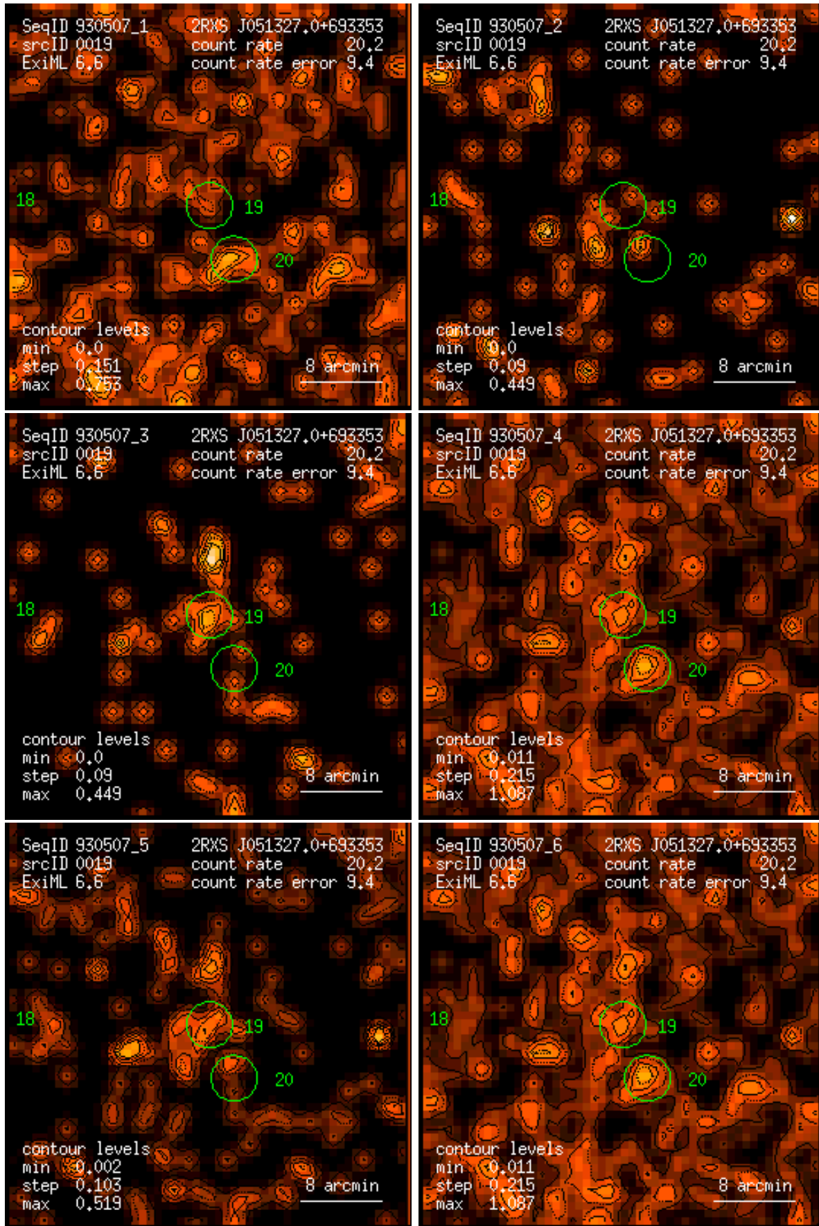
Figure 19: RASS 930507: detection 0019: band rate images, Gaussian filter: (1) PSPC channels 11 – 41, (2) 52 – 90, (3) 91 – 201, (4) 11 – 235, (5) 52 – 201, (6) 11 – 201. Broad band rates in counts/ks. Band rate contour levels in counts/ks/arcmin 2 .
