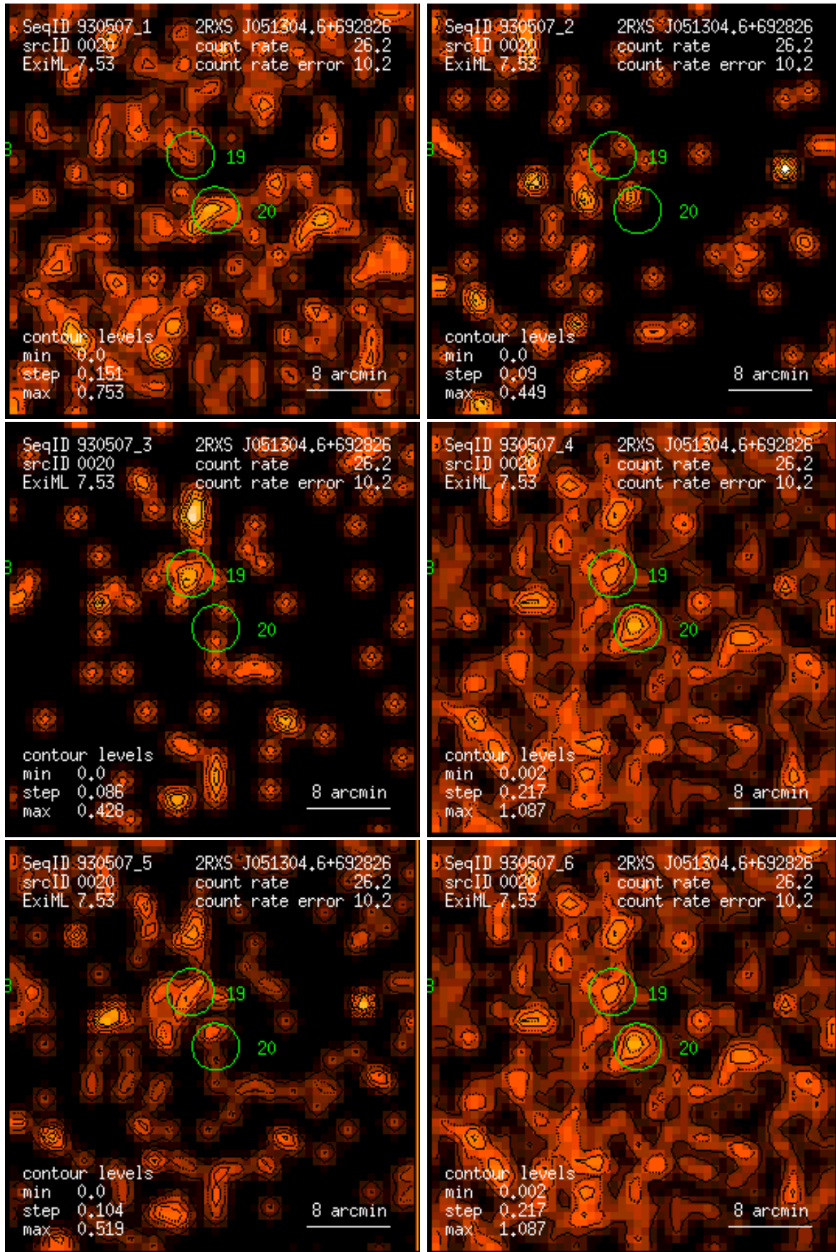
Figure 20: RASS 930507: detection 0020: band rate images, Gaussian filter: (1) PSPC channels 11 – 41, (2) 52 – 90, (3) 91 – 201, (4) 11 – 235, (5) 52 – 201, (6) 11 – 201. Broad band rates in counts/ks. Band rate contour levels in counts/ks/arcmin 2 .
