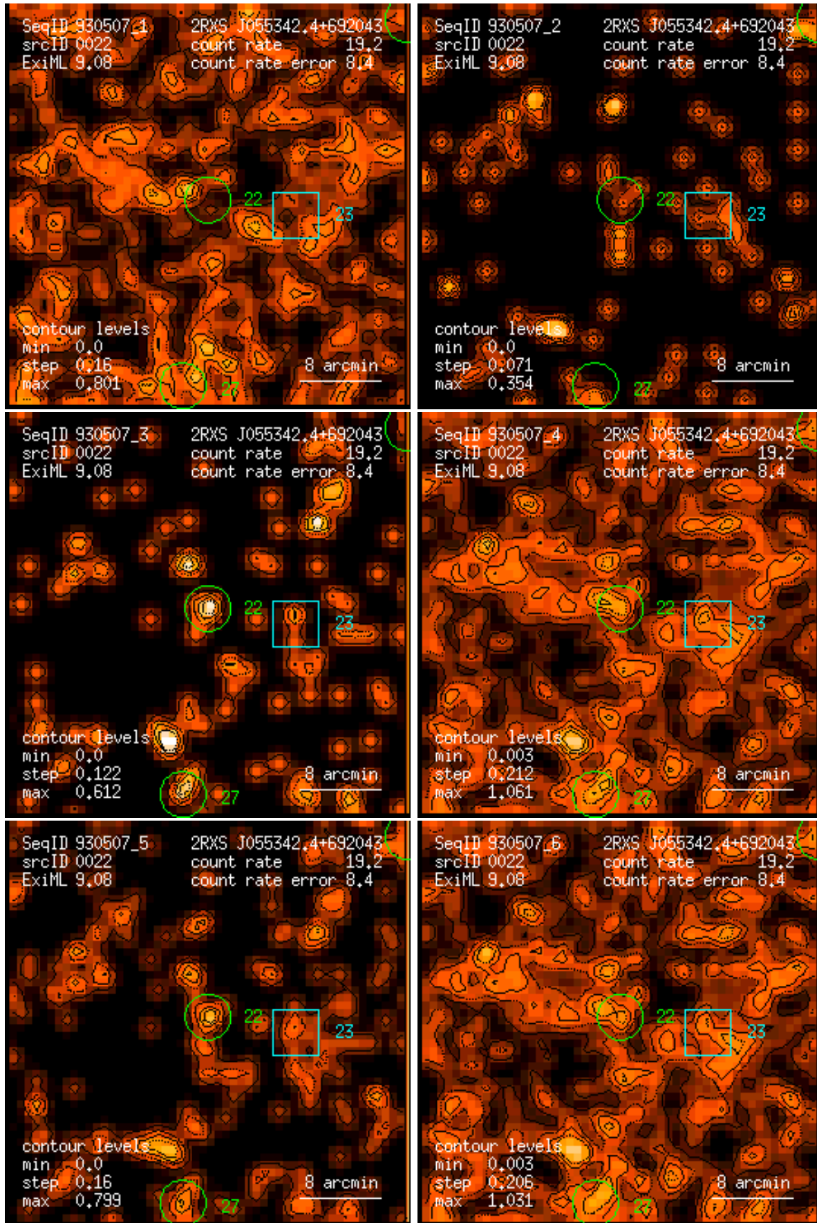
Figure 22: RASS 930507: detection 0022: band rate images, Gaussian filter: (1) PSPC channels 11 – 41, (2) 52 – 90, (3) 91 – 201, (4) 11 – 235, (5) 52 – 201, (6) 11 – 201. Broad band rates in counts/ks. Band rate contour levels in counts/ks/arcmin 2 .
