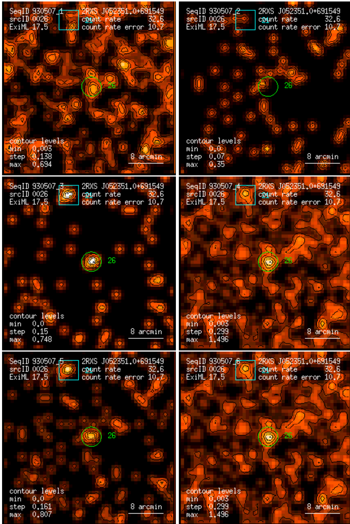
Figure 26: RASS 930507: detection 0026: band rate images, Gaussian filter: (1) PSPC channels 11 – 41, (2) 52 – 90, (3) 91 – 201, (4) 11 – 235, (5) 52 – 201, (6) 11 – 201. Broad band rates in counts/ks. Band rate contour levels in counts/ks/arcmin 2 .
