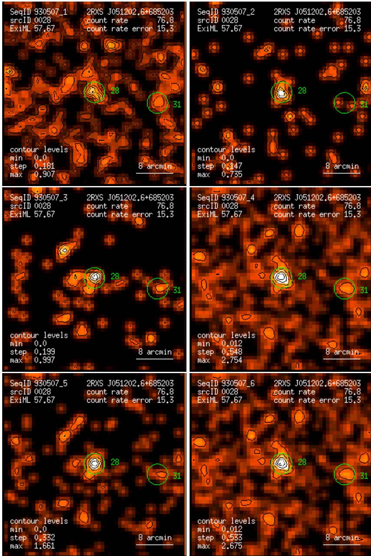
Figure 28: RASS 930507: detection 0028: band rate images, Gaussian filter: (1) PSPC channels 11 – 41, (2) 52 – 90, (3) 91 – 201, (4) 11 – 235, (5) 52 – 201, (6) 11 – 201. Broad band rates in counts/ks. Band rate contour levels in counts/ks/arcmin 2 .
