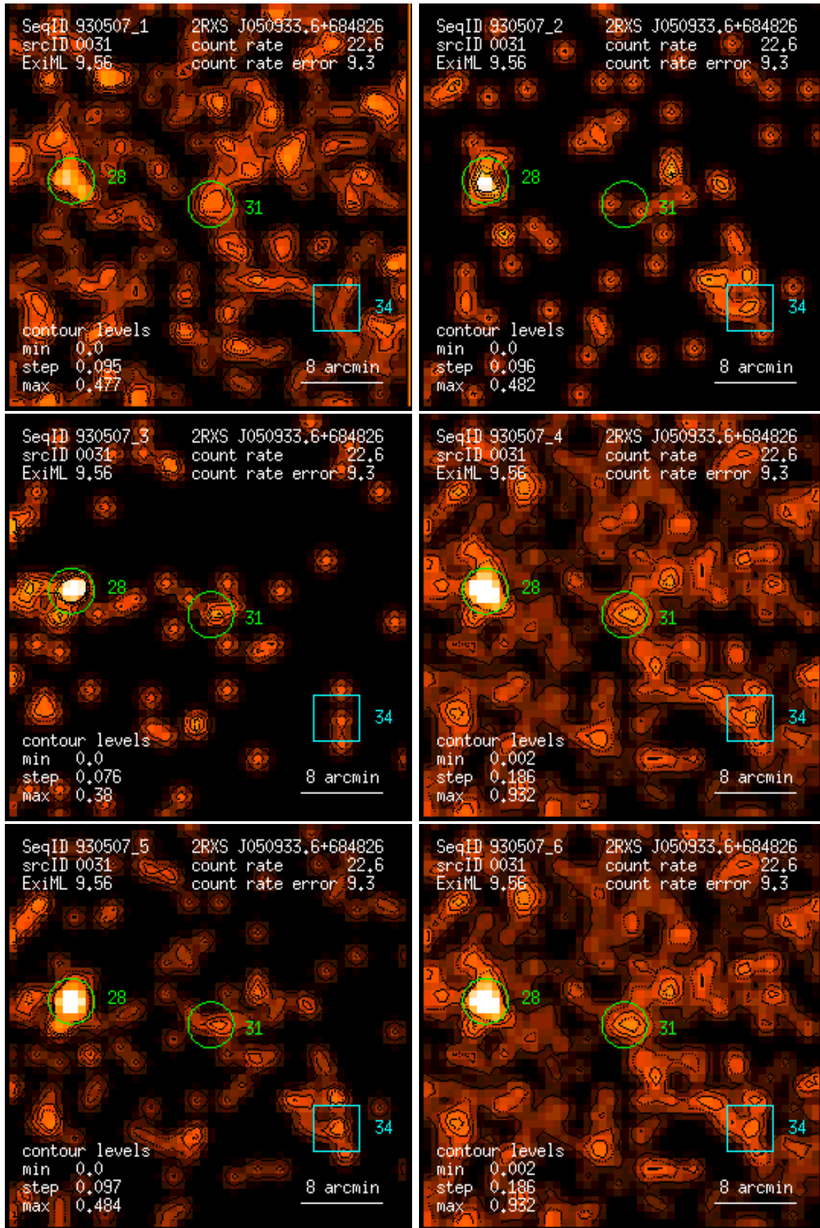
Figure 31: RASS 930507: detection 0031: band rate images, Gaussian filter: (1) PSPC channels 11 – 41, (2) 52 – 90, (3) 91 – 201, (4) 11 – 235, (5) 52 – 201, (6) 11 – 201. Broad band rates in counts/ks. Band rate contour levels in counts/ks/arcmin 2 .
