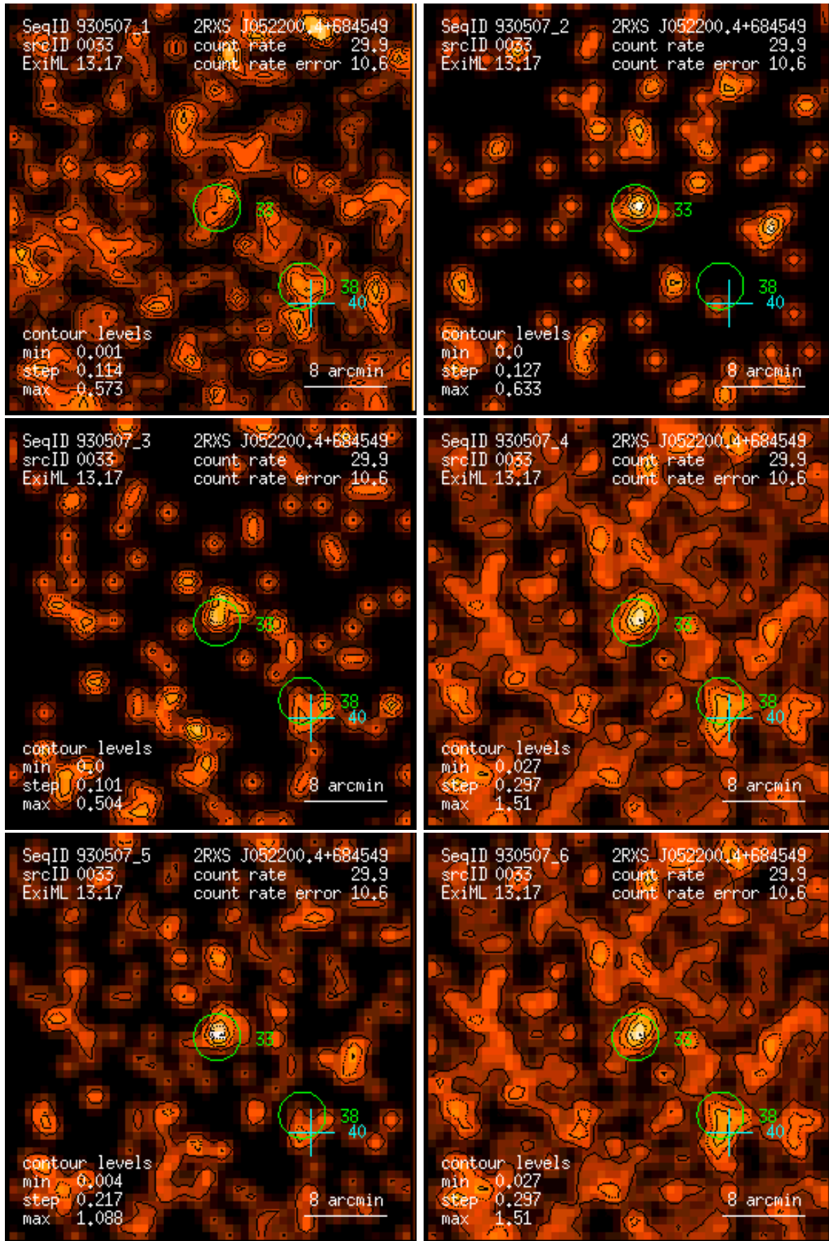
Figure 33: RASS 930507: detection 0033: band rate images, Gaussian filter: (1) PSPC channels 11 – 41, (2) 52 – 90, (3) 91 – 201, (4) 11 – 235, (5) 52 – 201, (6) 11 – 201. Broad band rates in counts/ks. Band rate contour levels in counts/ks/arcmin 2 .
